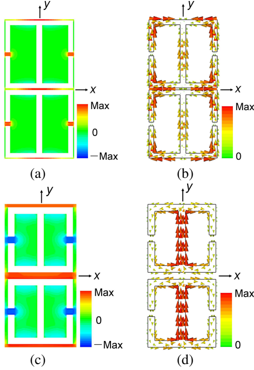
Figure 2. The distributions of (a) electric field component E_y and (b) surface current on the ELCs in dipole resonant mode. The distributions of (c) electric field component E_y and (d) surface current on the ELCs in LC resonant mode.
