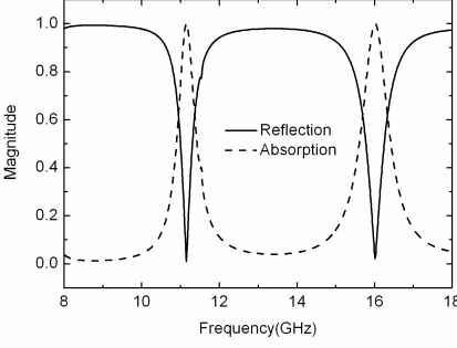
Figure 3. Simulated reflection and absorption as a function of frequency under normal incidence with electric field polarized along x axis.
