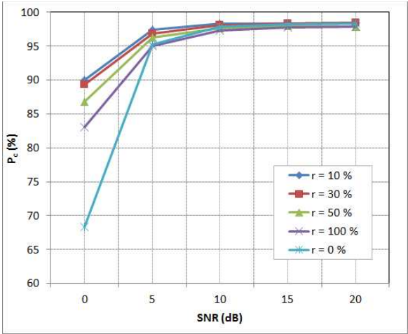
Figure 4. P_c versus SNR. 2DPCA-dimension = 2.
