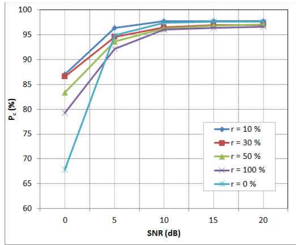
Figure 5. P_c versus SNR. 2DPCA-dimension = 3.
