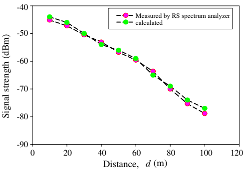
Figure 10. Measurements of signal strength of RFID tag.
