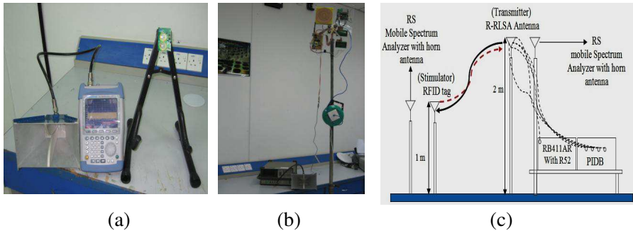
Figure 4. Measurement setup at (a) Measurements point. (b) Base station. (c) Graphical setup.
