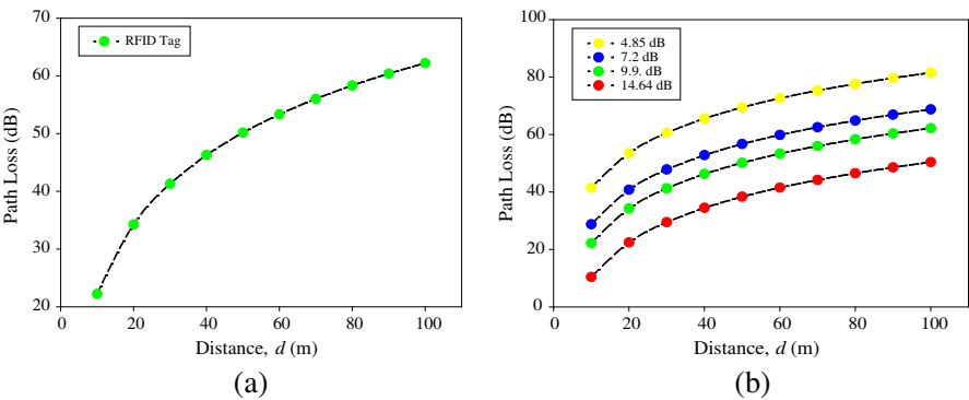
Figure 9. Calculated path loss (a) RFID tag, (b) R-RLSA antenna at base station.
