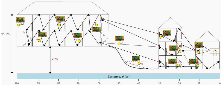
Figure 7. Measurement points of test-bay buildings model with RFID tag.
