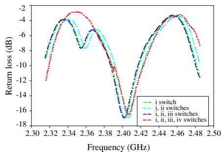
Figure 8. Return loss of R-RLSA antenna with copper tape.
