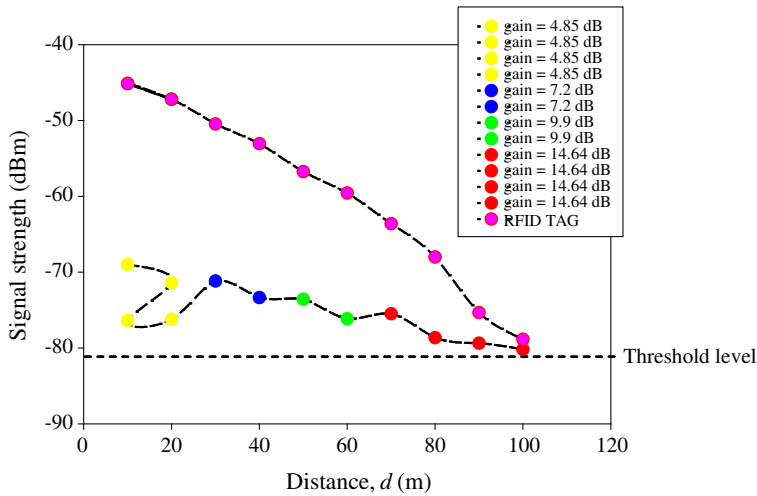
Figure 12. Signal strength measurements of the base station after activation of RFID tag.
