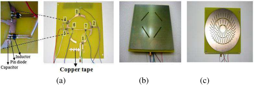
Figure 2. The reconfigurable beam shaped antenna [1], (a) feed line with PIN diode switches, (b) aperture slots, (c) RLSA radiating surface.
