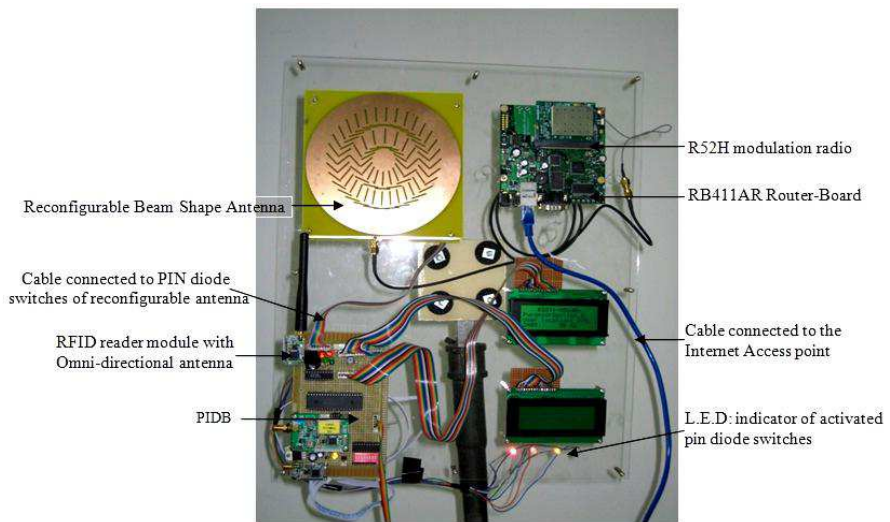
Figure 5. Complete prototype of adaptive Wi-Fi system.
