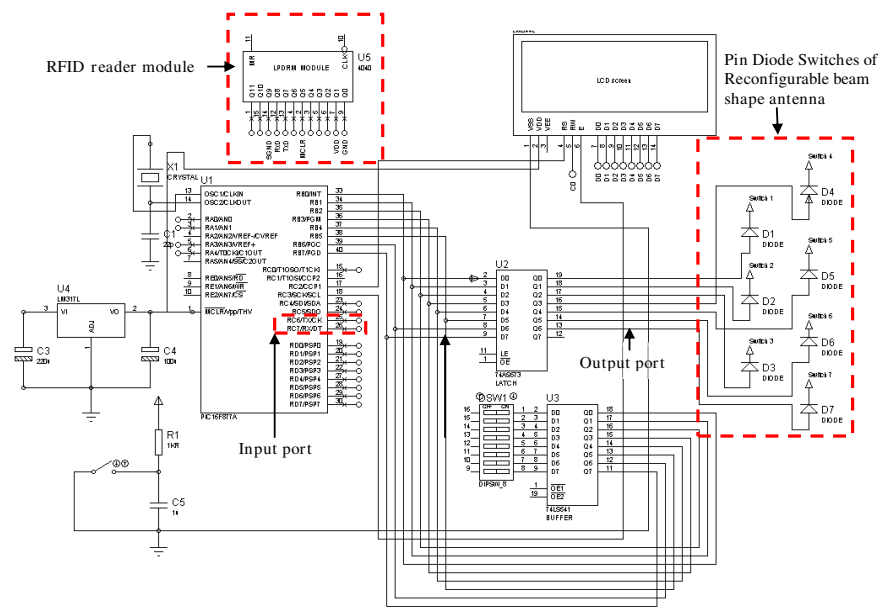
Figure 3. The schematic of Integration RFID technology and R-RLSA antenna into PIC Development Board (PIDB).
