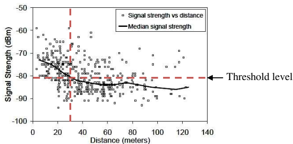
Figure 1. Wi-Fi signal strength over distance [14].
