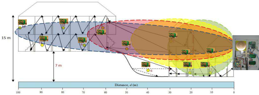
Figure 13. Illustration of adaptive Wi-Fi system using RFID tag.
