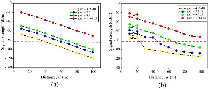
Figure 11. Signal strength of R-RLSA antenna (a) calculated, (b) measured.
