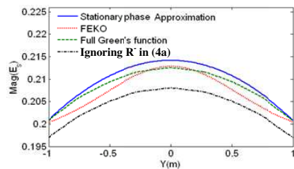
Figure 4. Scattered electric field from the circular cylinder.
