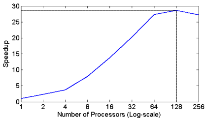
Figure 13. Speedup vs. the number of processors.
