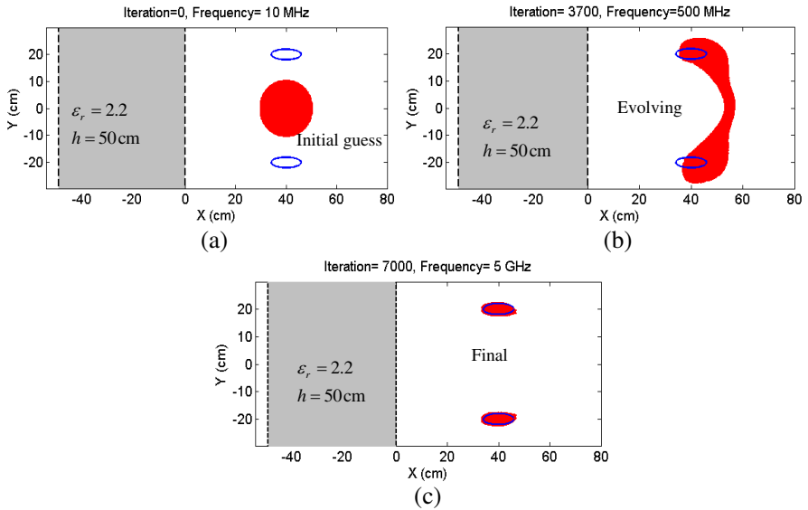
Figure 6. Reconstruction of two elliptical cylinders behind the dielectric wall when ( d = 40 cm). (a) Initial guess, (b) after 3700 iterations, (c) after 7000 iterations.
