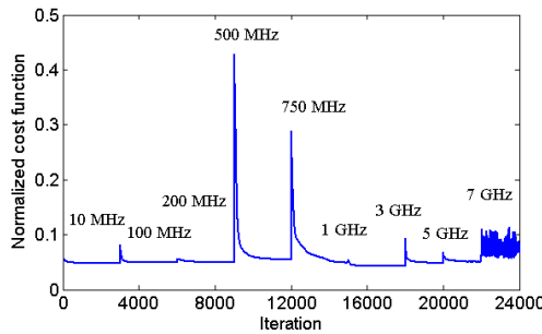
Figure 11. Normalized cost function for reconstruction of the three objects ( \text{SNR} = 10 \text{ dB} ).
