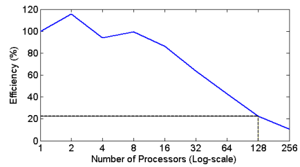
Figure 14. Efficiency vs. number of processors.
