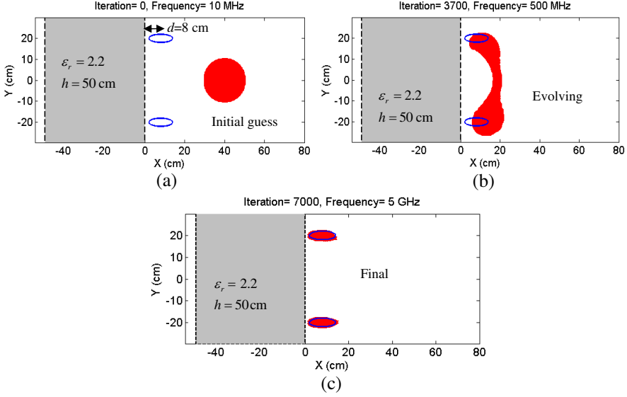
Figure 8. Reconstruction of two elliptical cylinders behind the dielectric wall when ( d = 8 cm). (a) Initial guess, (b) after 3700 iterations, (c) after 7000 iterations.
