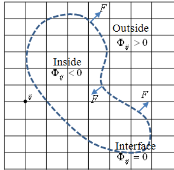
Figure 1. Implicit representation of the evolving contour using level set.
