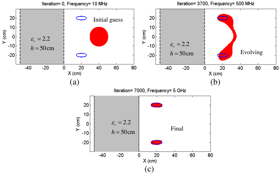
Figure 7. Reconstruction of two elliptical cylinders behind the dielectric wall when ( d = 20 cm). (a) Initial guess, (b) after 3700 iterations, (c) after 7000 iterations.
