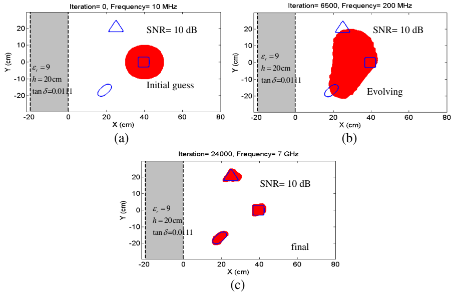
Figure 12. Noisy data of SNR = 10 dB. (a) Initial guess, after (b) 6500 iterations and (c) 24000 iterations.
