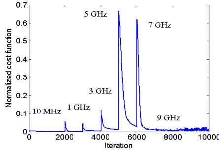
Figure 9. Normalized cost function for reconstruction of the defected pipe ( d = 60 cm).
