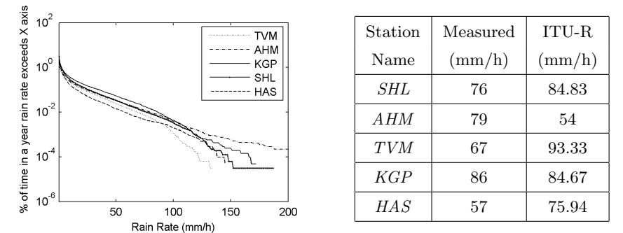
Figure 5. Rain rate exceedance probability for different locations. Table 4. Rain rate exceedance of 0.01% probability level.
