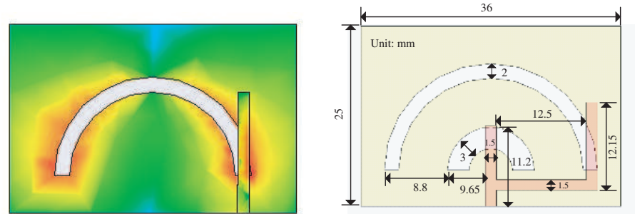
Figure 3. The surface current distribution fed by edge feeding method.
