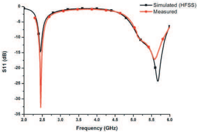
Figure 7. Measured and simulated parameters of S_{11} .
