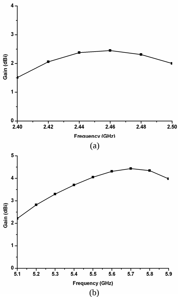
Figure 9. Measured peak gain of the antenna at dual bands. (a) Low band (2.4–2.484 GHz); (b) High band (5.15–5.825 GHz).
