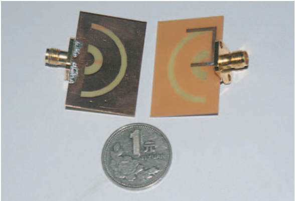
Figure 6. Photograph of the proposed antenna.
