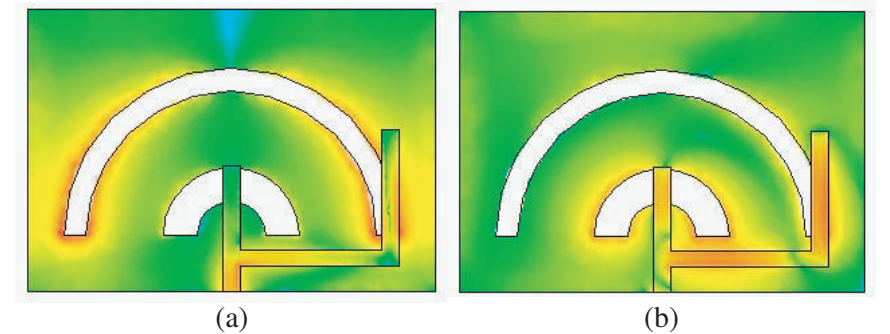
Figure 5. The surface current distribution at (a) 2.45 GHz; (b) 5.5 GHz.
