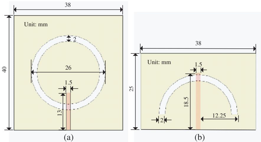
Figure 1. The geometry of (a) Conventional circular loop slot antenna; (b) Inverted C-shaped slot antenna.
