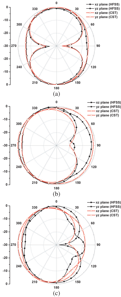
Figure 8. Radiation patterns of the proposed antenna simulated by Ansoft HFSS and CST STUDIO. (a) 2.4 GHz; (b) 5.2 GHz; (c) 5.8 GHz.
