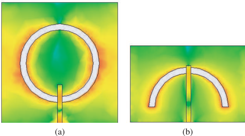
Figure 2. The magnitude of the surface current distribution. (a) Conventional circular loop slot antenna; (b) Inverted C-shaped slot antenna.
