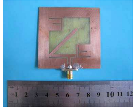
Figure 13. Fabricated broadband circularly polarized antenna.
