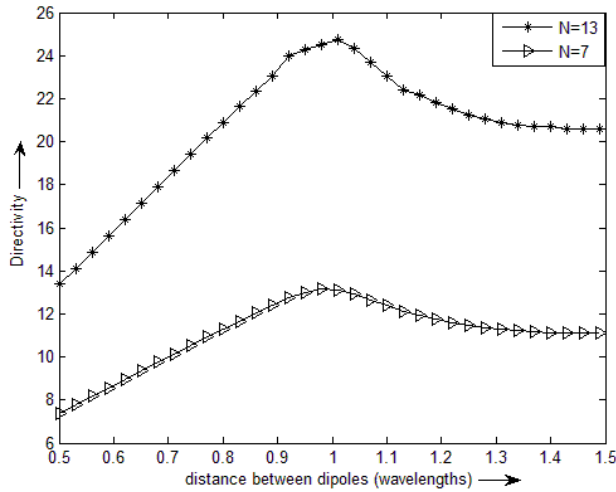
Figure 10. Directivity of a collinear array of half wavelength dipoles as a function of the distance between the dipoles.
