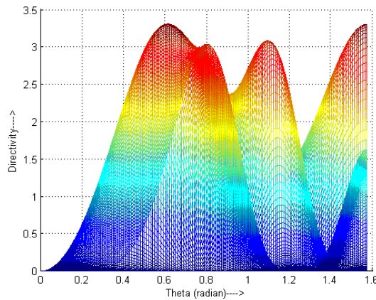
Figure 6. Projection of the directivity of the dipole onto the observation angle-directivity plane.
