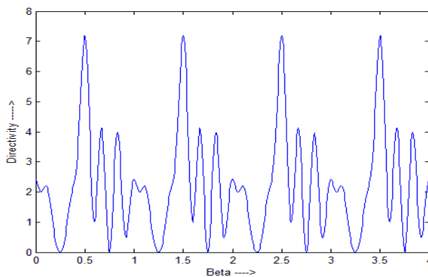
Figure 12. Directivity of a circular array of eight dipoles as a function of \beta for \theta = \pi/2 , \phi = 0 .
