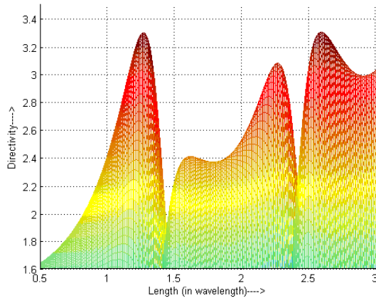
Figure 5. Projections of the directivity of a dipole onto the length-directivity plane.
