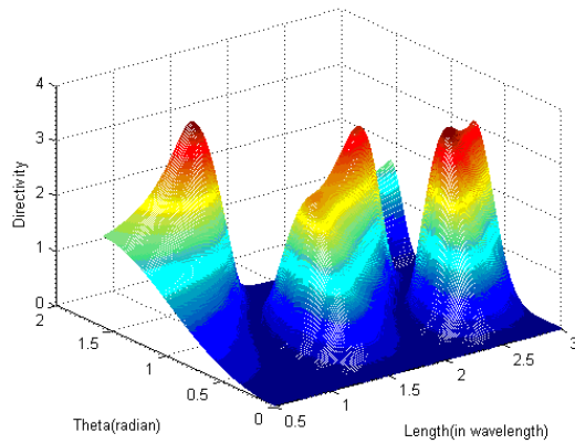
Figure 4. Directivity of a dipole versus it's length and the observation angle.
