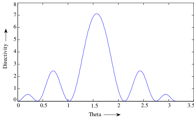
Figure 13. Directivity of a circular array of eight dipoles as a function of \theta for \beta = 2 , \phi = 0 .
