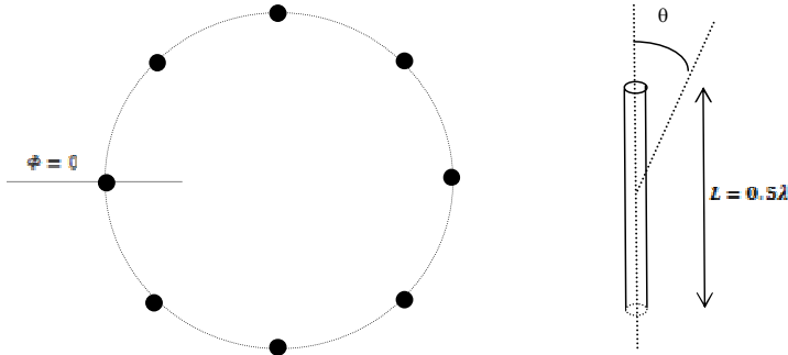
Figure 11. Circular array of 8 half-wavelength dipoles.
