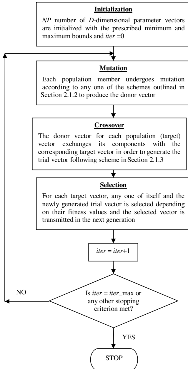
Figure 1. Flowchart for the differential evolution algorithm.
