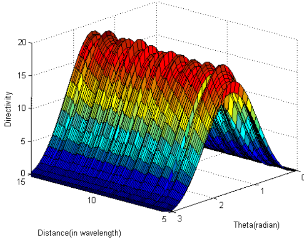
Figure 8. Directivity of a uniform linear array of half wavelength dipoles as a function of the spacing between the elements and the observation angle.
