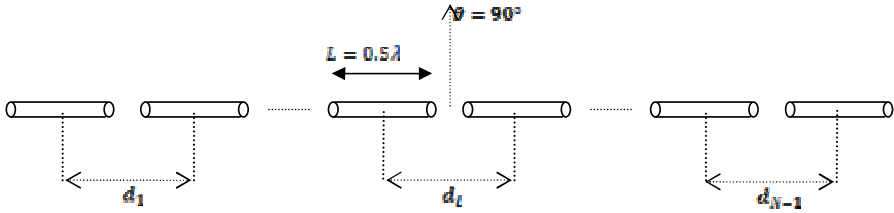
Figure 9. Collinear array of N half-wavelength long dipoles.
