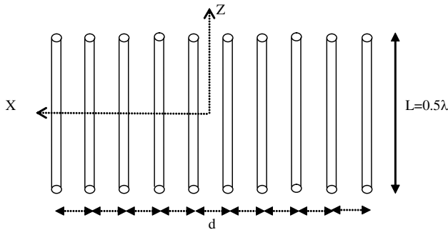
Figure 7. Uniform linear array of half wavelength dipoles.
