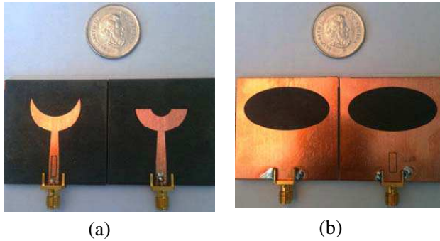
Figure 18. Fabricated band-notched antenna prototypes A and B (a) top, (b) bottom.
