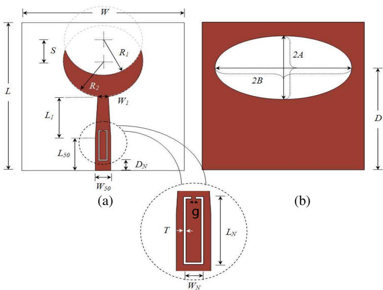
Figure 10. The geometry of the proposed antenna B (a) front view, (b) back view.
