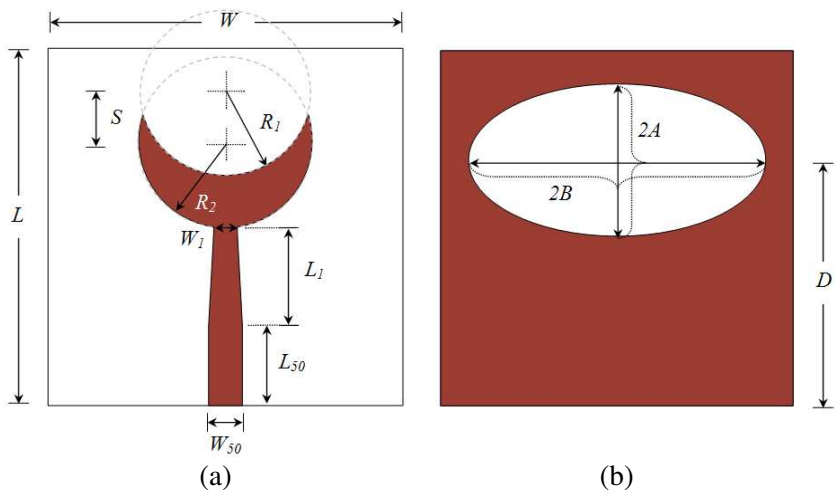
Figure 4. Geometry of the proposed antenna prototype #B design (a) top view, (b) bottom view.
