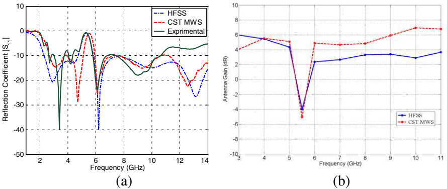
Figure 11. Measured and simulated (a) reflection coefficient S_{11} , (b) gain curves of the proposed antenna A.
