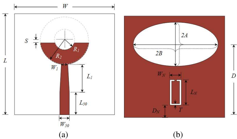
Figure 9. The geometry of the proposed antenna A (a) front view, (b) back view.
