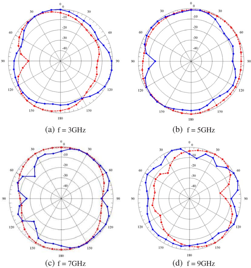
Figure 6. Calculated E -plane (red dashed) and H -plane (blue solid) radiation patterns for the proposed antenna prototype #B at (a) 3 GHz, (b) 5 GHz, (c) 7 GHz and (d) 9 GHz.
