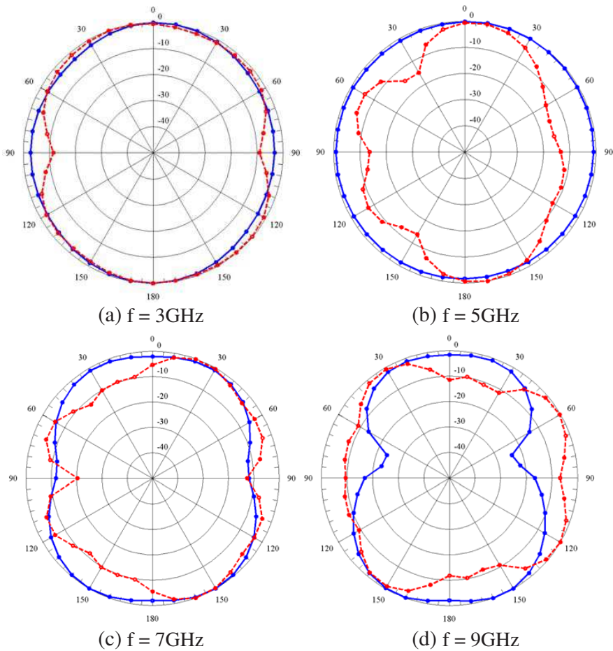
Figure 13. Calculated E -plane (red dashed) and H -plane (blue solid) radiation patterns for proposed antenna prototype #A at (a) 3 GHz (b) 5 GHz (c) 7 GHz and (d) 9 GHz.
