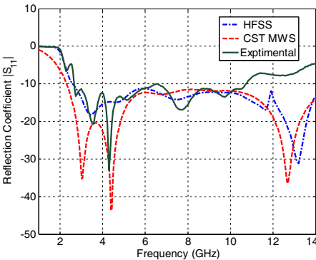
Figure 2. Simulated and experimental return loss S_{11} of the proposed antenna prototype #A design.
