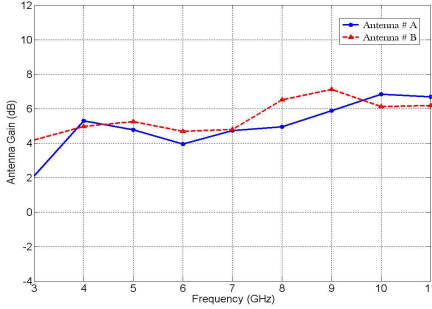
Figure 7. Calculated gain curves for the proposed antenna prototypes #A and B.
