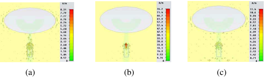
Figure 15. Surface current for proposed antenna prototype #A at (a) 3 GHz, (b) 5.5 GHz and (d) 9 GHz.
