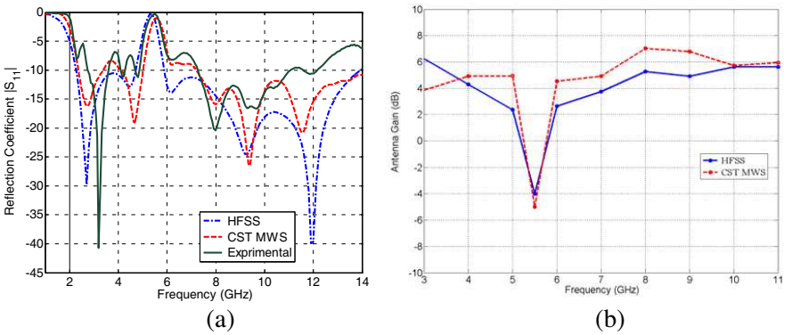
Figure 12. Measured and simulated (a) reflection coefficient S_{11} , (b) gain curves of the proposed antenna B.
