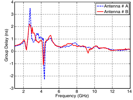
Figure 8. Measured group delay for the proposed antenna prototypes #A and B.
