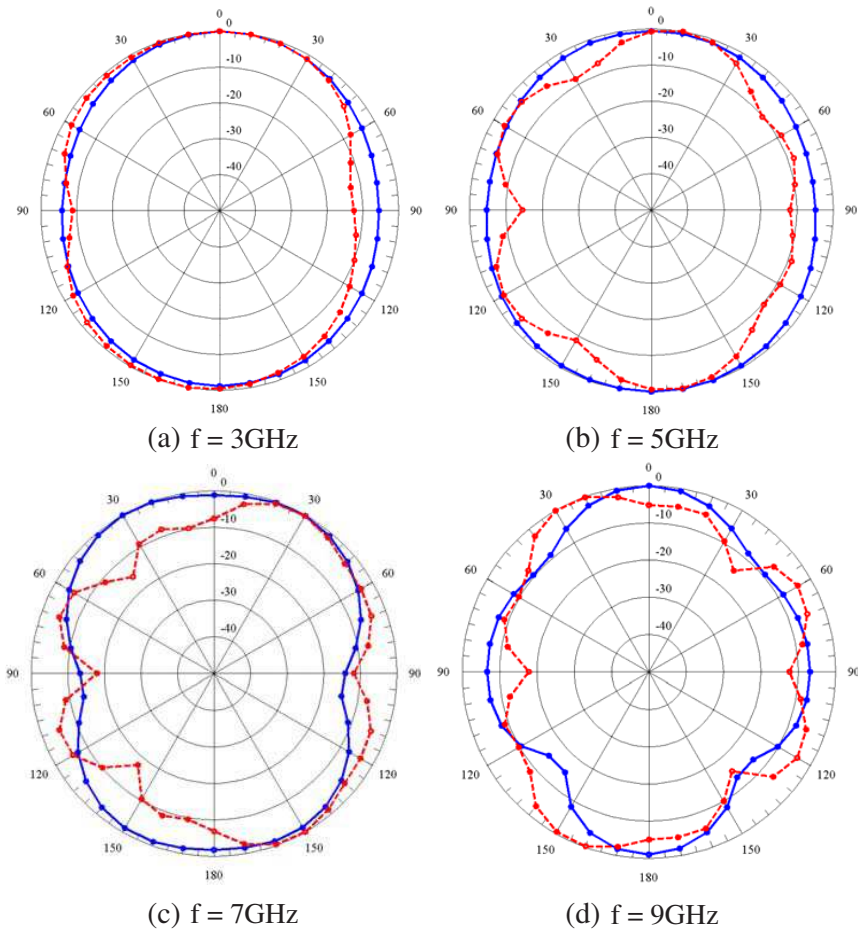
Figure 14. Calculated E -plane (red dashed) and H -plane (blue solid) radiation patterns for proposed antenna prototype #B at (a) 3 GHz, (b) 5 GHz, (c) 7 GHz and (d) 9 GHz.
