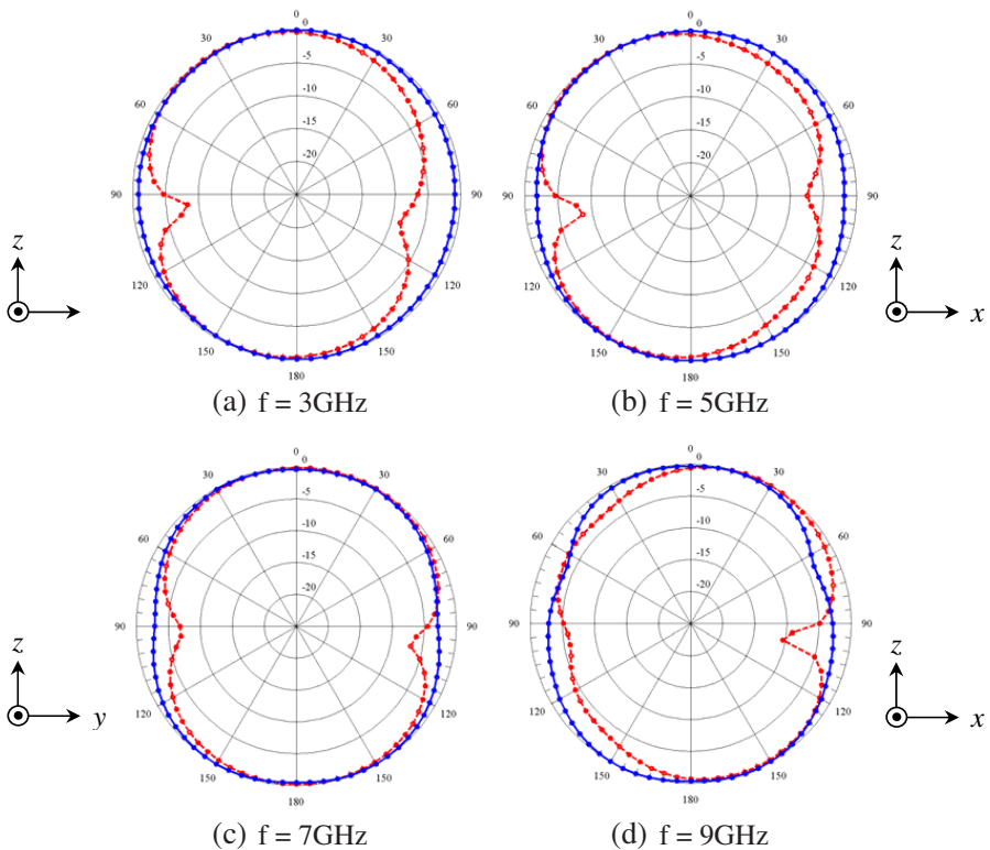
Figure 3. Calculated E -plane (red dashed) and H -plane (blue solid) radiation patterns for proposed antenna prototype #A at (a) 3 GHz, (b) 5 GHz, (c) 7 GHz and (d) 9 GHz.
