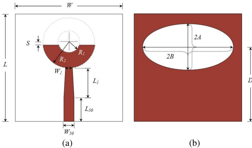
Figure 1. Geometry of the proposed antenna prototype #A design (a) top view, (b) bottom view.
