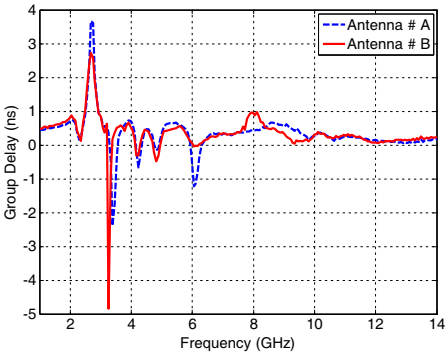
Figure 17. Measured group delay for the proposed band-notched antenna prototypes #A and B.
