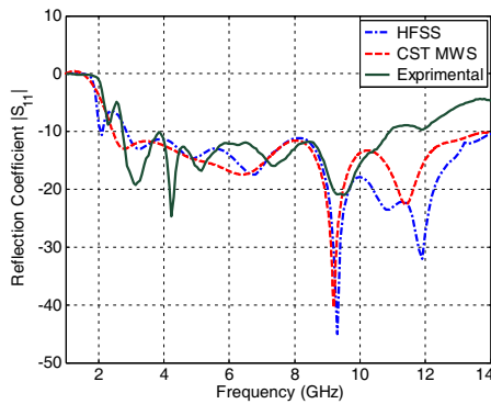
Figure 5. Simulated and experimental return loss S_{11} of the proposed antenna prototype #B design.
