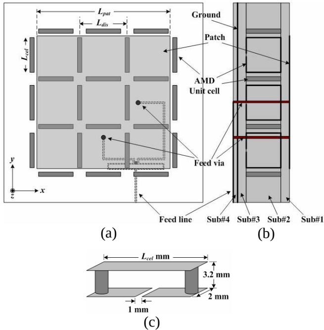
Figure 1. The proposed antenna structure in (a) top view, (b) side view, and (c) a unit cell.
