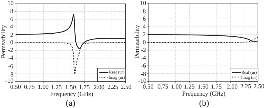
Figure 3. Permeability of AMD structure with (a) x -axis array and (b) y -axis array.
