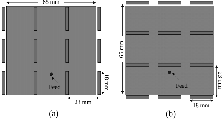
Figure 2. Arrayed AMD structure (a) x -axis and (b) y -axis.
