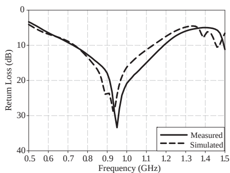
Figure 9. Measured and simulated return loss characteristics.
