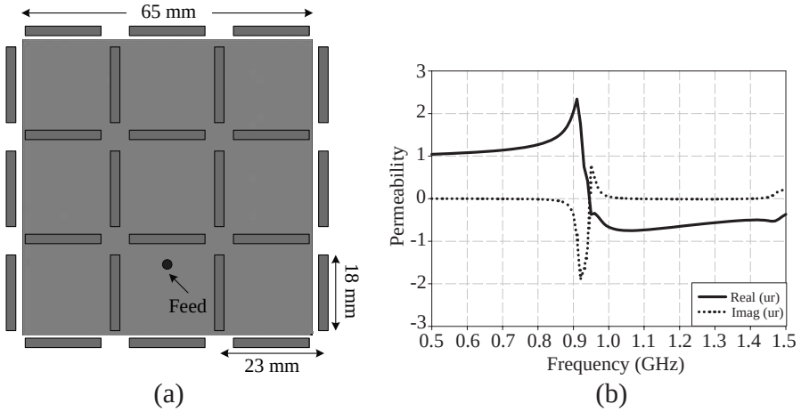
Figure 4. 2-D arrayed AMD substrate (a) structure and (b) permeability.
