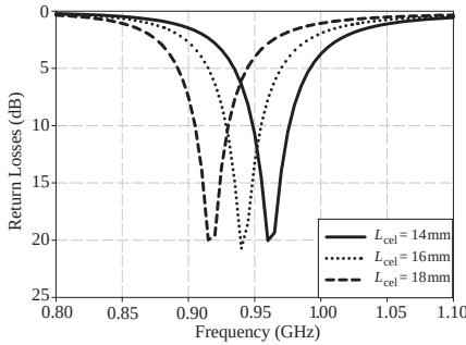
Figure 6. Return loss characteristics for various the length of a unit cell L_{\text{cel}} .
