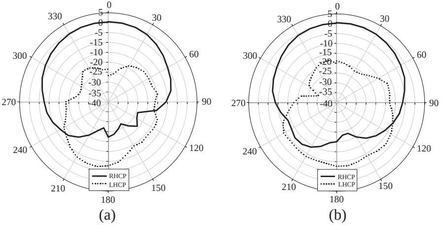
Figure 10. Measured radiation patterns (a) x - z plane and (b) y - z plane.
