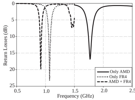
Figure 5. Return loss characteristics for three different substrates.
