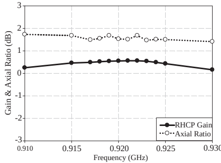
Figure 11. Measured peak gain and axial ratio.
