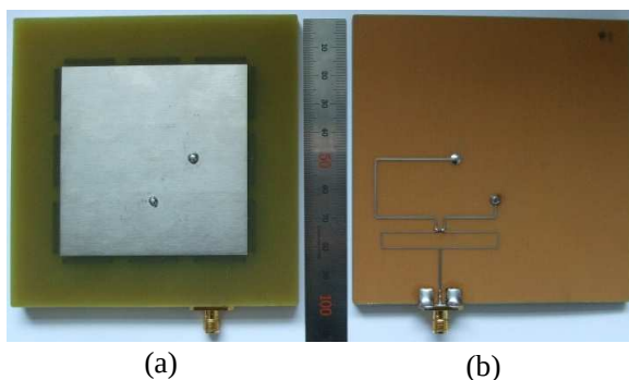
Figure 8. Photograph of the fabricated antenna (a) top view and (b) bottom view.
