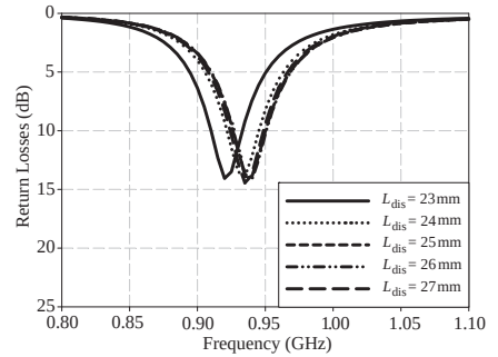
Figure 7. Return loss characteristics for the various distances between unit cells L_{\text{dis}} .
