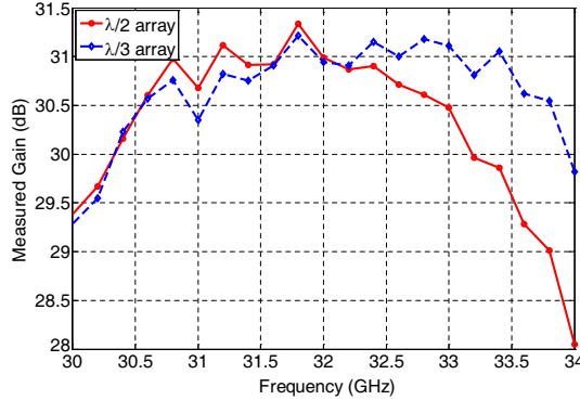
Figure 5. Measured gain of the fabricated reflectarrays. The 1 dB gain bandwidth is 8.0% for the \lambda/2 reflectarray and 10.9% for the \lambda/3 reflectarray.
