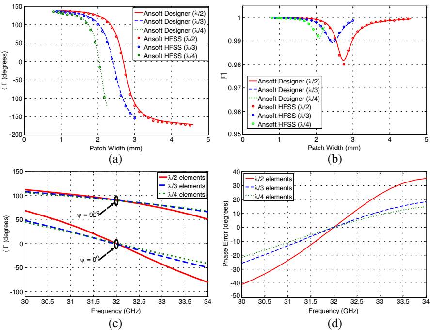
Figure 2. (a) Reflection phases versus patch size at the center frequency 32 GHz for \lambda/2 , \lambda/3 , and \lambda/4 unit-cells. (b) Reflection magnitude versus patch size at the center frequency 32 GHz for \lambda/2 , \lambda/3 , and \lambda/4 unit-cells. (c) Reflection phases versus frequency for 0^\circ and 90^\circ elements for \lambda/2 , \lambda/3 , and \lambda/4 unit-cells. (d) Phase errors for a 90^\circ relative phase difference versus frequency for \lambda/2 , \lambda/3 , and \lambda/4 unit-cells.
