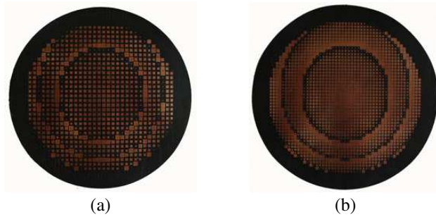
Figure 3. Photographs of the fabricated arrays. (a) \lambda/2 array with 848 square patches, (b) \lambda/3 array with 1941 square patches.
