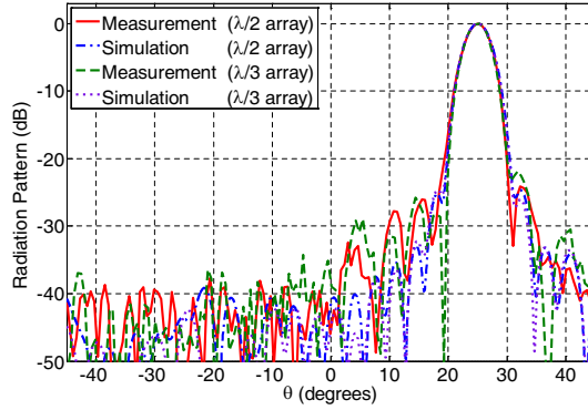
Figure 4. Measured and calculated radiation patterns of the antennas at 32 GHz.
