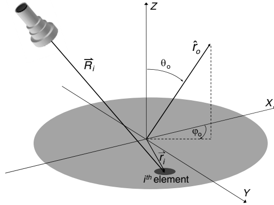
Figure 1. Geometry of the reflectarray antenna.
