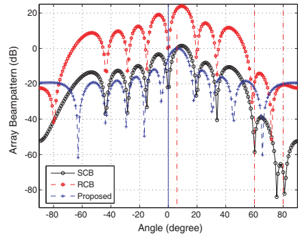
Figure 3. Comparison of the beampatterns of SCB, RCB and proposed method ( \Delta\theta = 6^\circ , SNR = 30 dB, INR_1 = INR_2 = 20 dB).
