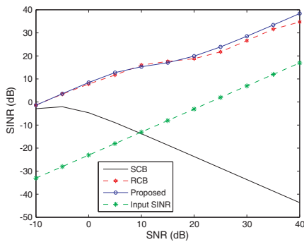
Figure 4. Comparison of the SINRs of SCB, RCB and proposed method ( \Delta\theta = 3^\circ , INR_1 = INR_2 = 20 dB).
