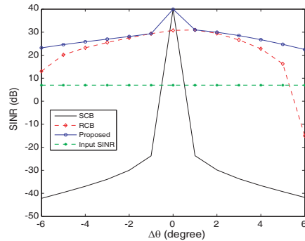
Figure 5. Comparison of the SINRs of SCB, RCB and proposed method ( SNR = 30 dB, INR_1 = INR_2 = 20 dB).
