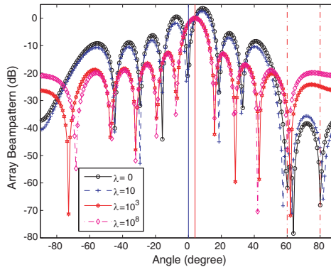
Figure 1. Comparison of the beampatterns of different diagonal loading levels ( \Delta\theta = 4^\circ ).
