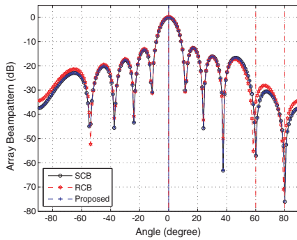
Figure 2. Comparison of the beampatterns of SCB, RCB and proposed method ( \Delta\theta = 0 , SNR = 10 dB, INR_1 = INR_2 = 20 dB).
