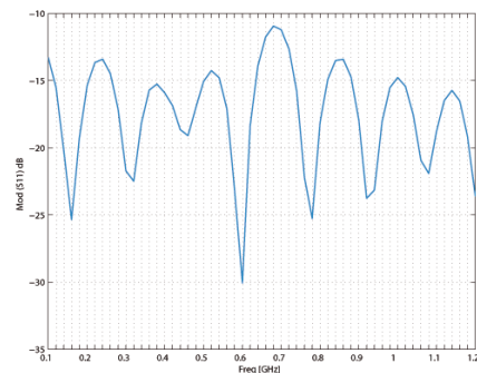
Figure 5. Frequency response of the reflection coefficient at the feed unbalanced port of the balun.
