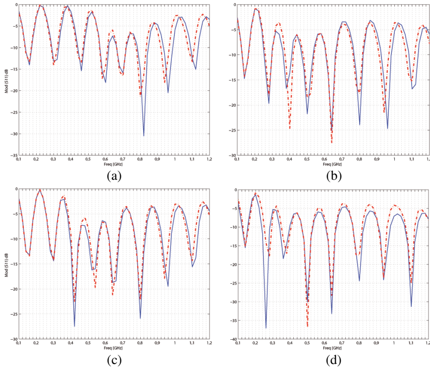
Figure 7. Frequency response of the Modulus of S_{11} at the feed port of balun (fed in unbalanced way by a coaxial cable). Blu line: Monolithic antenna; Red line: Discretised reconfigurable antenna. (a) Antenna in free-space. (b) Antenna on half space with relative dielectric permittivity 4. (c) Antenna on half-space with relative dielectric permittivity 9. (d) Antenna on half-space with relative dielectric permittivity 16.
