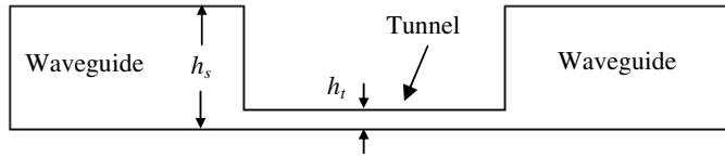
Figure 1. Schematic of the Epsilon Near Zero approach using waveguide technology.
