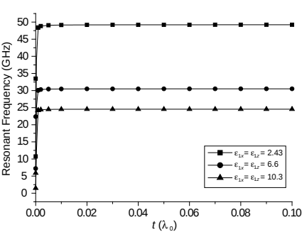
Figure 2. The resonant frequency versus the thickness of patch ( \sigma_n = 210\text{s/mm} , \lambda_0 = 1500\text{ \AA} and T/T_c = 0.5 , a = 1\text{ mm} , d_1 = 1.2\text{mm} ).
