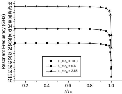
Figure 3. The resonant frequency versus the normalized temperature ( \sigma_n = 210\text{s/mm} , \lambda_0 = 1500\text{ \AA} and t_c = 89^\circ , a = 1\text{ mm} , d_1 = 1.2\text{ mm} and t = 0.02\text{ }\mu\text{m} ).
