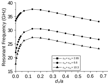
Figure 8. Resonant frequency versus the air separation, for circular microstrip antenna for three dielectric constant: \varepsilon_{2x} = \varepsilon_{2z} = 2.65 , \varepsilon_{2x} = \varepsilon_{2z} = 6.6 , and \varepsilon_{2x} = \varepsilon_{2z} = 10.3 , a = 1.5 mm. \sigma_n = 210 s/mm, \lambda_0 = 1500 Å, and T/T_c = 0.5 , and t = 0.02 μm.
