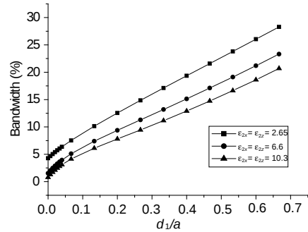
Figure 9. Bandwidth versus the air separation, for circular microstrip antenna for three dielectric constant: \varepsilon_{2x} = \varepsilon_{2z} = 2.65 , \varepsilon_{2x} = \varepsilon_{2z} = 6.6 , and \varepsilon_{2x} = \varepsilon_{2z} = 10.3 , a = 1.5 mm. \sigma_n = 210 s/mm, \lambda_0 = 1500 Å, and T/T_c = 0.5 , and t = 0.02 μm.
