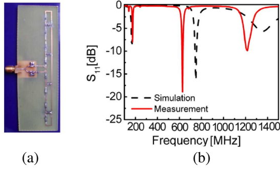
Figure 2. (a) Picture of the prototype. (b) Simulated and measured return loss for the 4 unit cell left-handed dipole.
