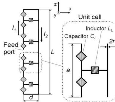
Figure 1. Model of the dipole antenna with left-handed transmission line. Dipole parameters are C_L = 2.3 pF, L_L = 280 nH, a = 25 , d = 10 and r = 0.7 . Units are in mm.
