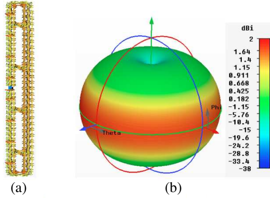
Figure 3. (a) Current distribution, and (b) 3D far field radiation pattern at 750 MHz n = 0 mode.
