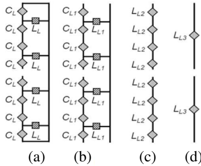
Figure 4. Different antenna configurations. (a) Left-handed dipole with shorted ends, (b) left-handed dipole, (c) right-handed dipole with lumped inductors at periodic intervals, (d) right-handed dipole with two lumped inductors. Element values are C_L = 2.3 pF, L_L = 280 nH, C_{L1} = 113 pF, L_{L1} = 22 nH, L_{L2} = 16.5 nH, and L_{L3} = 53 nH.
