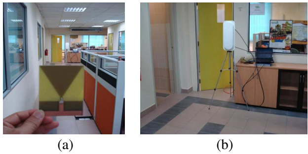
Figure 9. Measurement setup (a) receiver (RFID tag), (b) transmitter (RFID reader).
