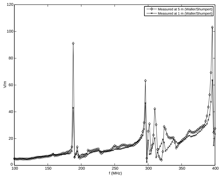
Figure 10. Measured aperture fields, horizontal/ TM .
