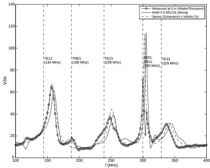
Figure 7. “Spatially averaged” internal fields, vertical/ TE .
