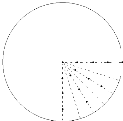
Figure 2. Cylinder cross section with internal and aperture probe positions.
