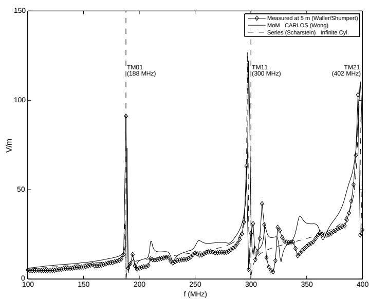
Figure 6. Aperture fields, horizontal/ TM .
