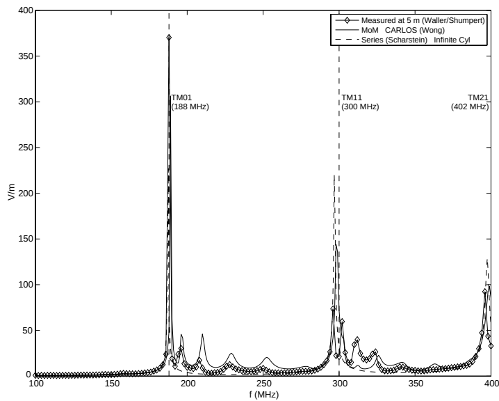
Figure 8. “Spatially averaged” internal fields, horizontal/ TM .
