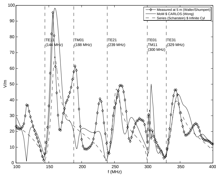
Figure 5. Aperture fields, vertical/ TE .
