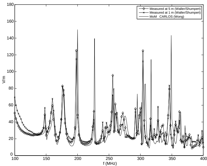
Figure 13. “Spatially averaged” internal fields, vertical/ TE , “shorted cylinder.”
