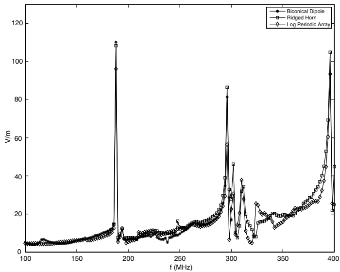
Figure 4. Measured aperture fields, horizontal/ TM .
