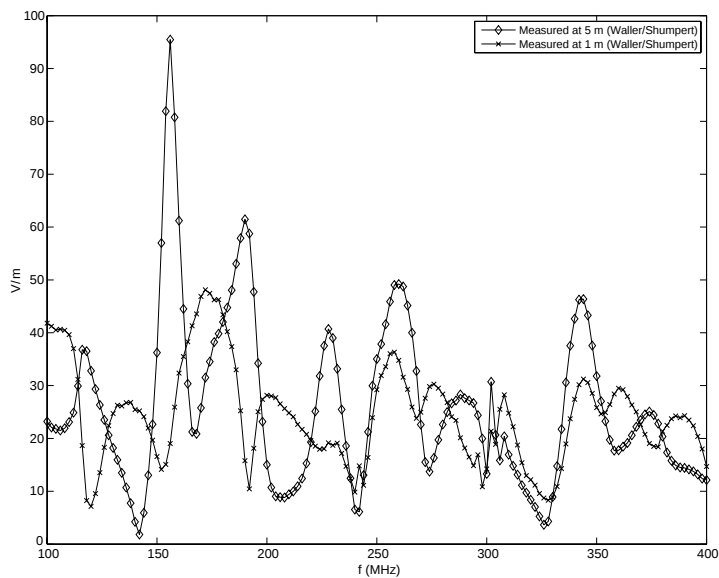
Figure 9. Measured aperture fields, vertical/ TE .
