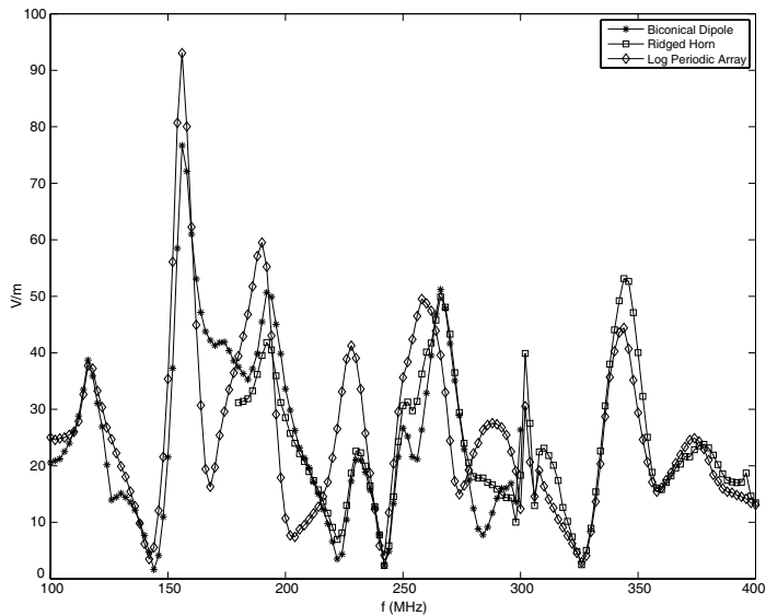
Figure 3. Measured aperture fields, vertical/ TE .
