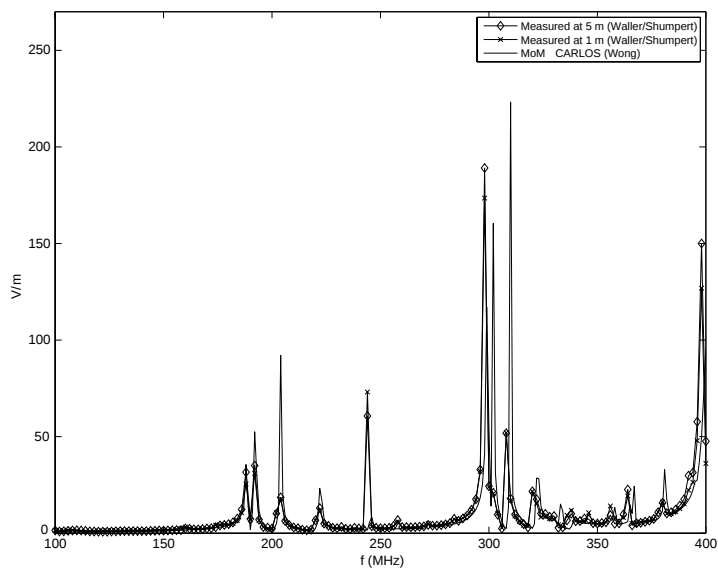
Figure 14. “Spatially averaged” internal fields, horizontal/ TM , “shorted cylinder.”
