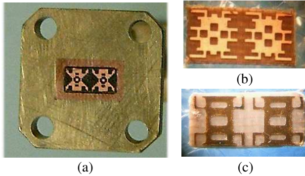
Figure 2. The composite material consists of two square cells with a side of 3.556 mm placed along the transverse direction of the Ka waveguide. (a) Picture of a sample accommodated in the waveguide. (b) Realized sample of the filter 2, and (c) filter 3.
