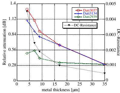
Figure 6. In-band relative attenuation as a function of the metal sheet thickness. Relative attenuation (Datt) is defined as the difference between the measured attenuation and the attenuation calculated by means of the simulation.
