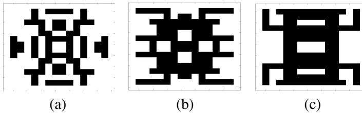
Figure 1. Unit cells of the three analyzed FSS filters. The FSS filter consists of two unit cells with periodicity of 3.556\text{ mm} . (a) filter 1, (b) filter 2, (c) filter 3.
