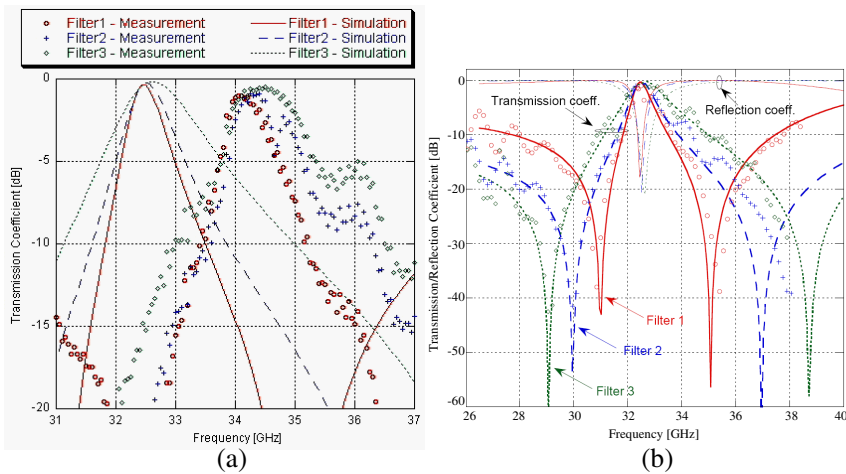
Figure 4. The transmission and reflection coefficient as a function of the frequency for three filter samples (1, 2 and 3) of the Batch A with t = 17\mu\text{m} , compared with the simulations. (a) Comparison between the original experimental (dotted) and simulated (line) TF. (b) Agreement between the measured and the simulated transfer function shape after rigid frequency shift of the former.
