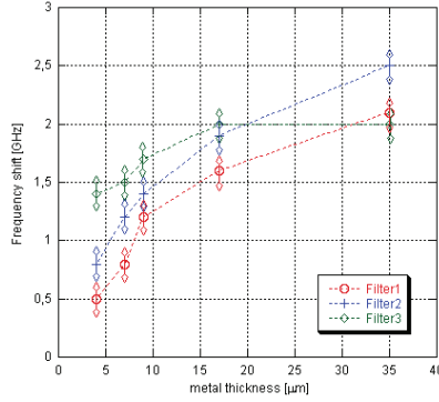
Figure 5. Frequency blueshift of the transfer functions of the filter sample 1, 2 and 3 of the batch A as a function of the metal sheet thickness.
