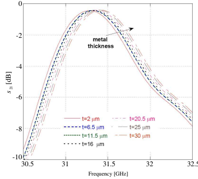
Figure 8. Computed transmission coefficients for different metal sheet thickness obtained by CST microwave studio simulations of the filter 2.
