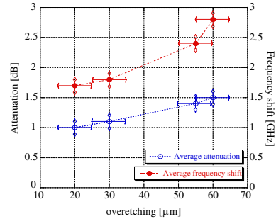
Figure 7. The average frequency shift and the attenuation of the filters 1, 2 and 3 of the batch B. While the attenuation is significantly affected by the size of the overetching, the effect on the frequency is small if compared to that due to the metal sheet thickness in the thickness range reported in Figure 5.
