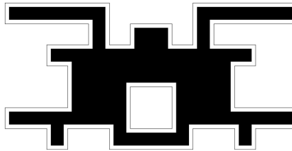
Figure 3. Overetching effect. The line indicates the nominal shape of the cell. The picture reports the unit cell of the filter 2 halved.
