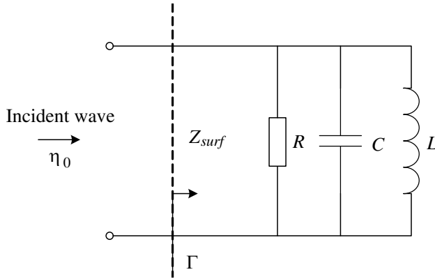
Figure 1. The absorbing equivalent circuit of high impedance surface.
