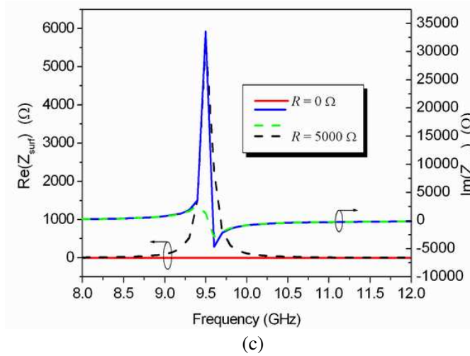
Figure 9. (a) Reflection coefficient amplitude of variation with load resistance R . (b) Reflection phase characteristics. (c) Surface equivalent impedance of variation with R .
