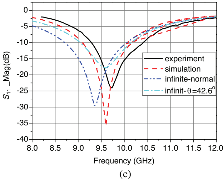
Figure 12. (a) Waveguide simulation model. (b) Test sample is mounted in the port of a waveguide, and a waveguide-coaxial adaptor for S_{11} measurement of the JCS absorber. (c) Comparison of measurement results with simulation results in waveguide model, in which the results calculated by using infinite periodic model for normal incidence and oblique incidence ( \theta = 42.6^\circ ) are also given for comparison.
