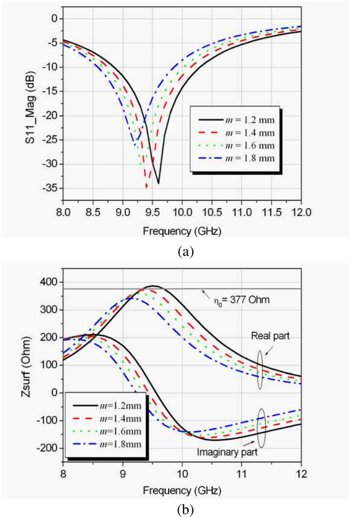
Figure 5. (a) Reflection coefficient curve. (b) Effective surface impedance of variation with JCS length m .
