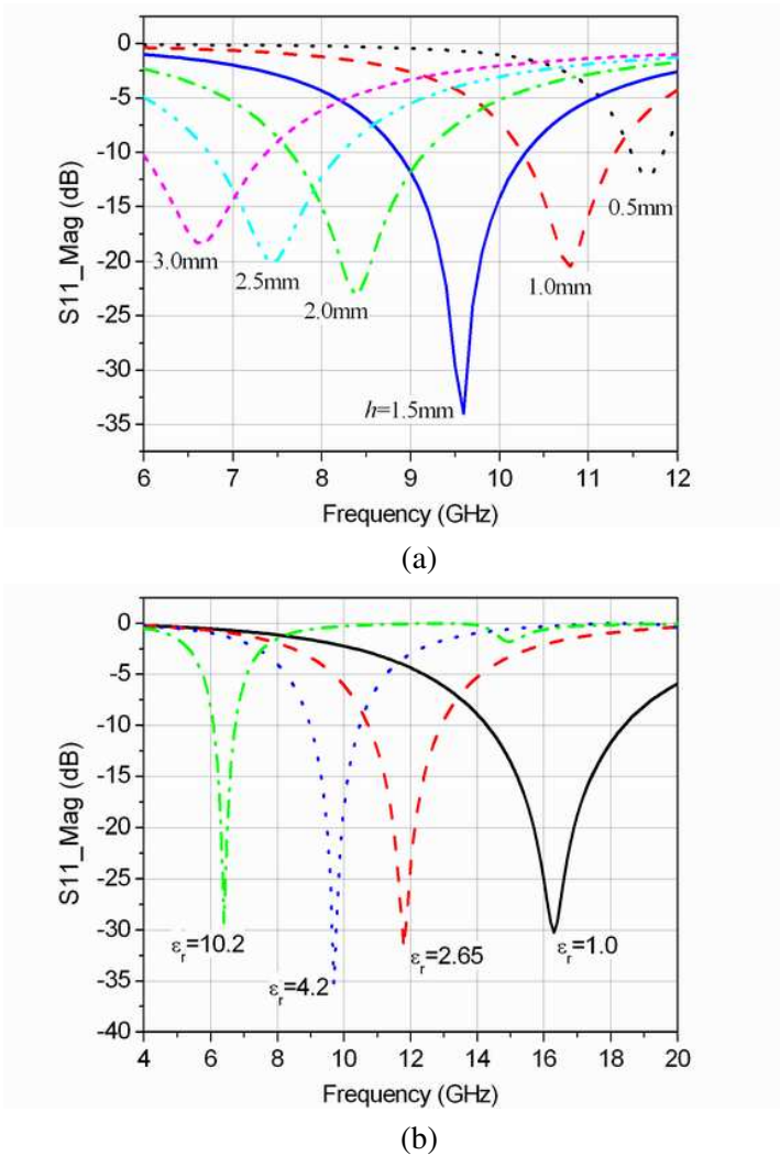
Figure 10. Reflection coefficient variation with (a) substrate thickness effect, (b) substrate permittivity effect.
