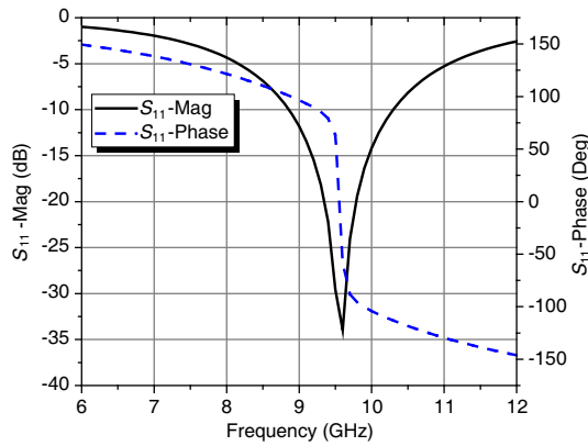
Figure 3. Reflection coefficient characteristics of Jerusalem cross slot absorbing structure versus frequency.
