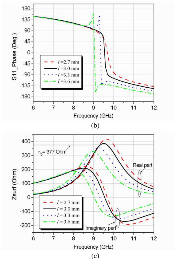
Figure 4. (a) Amplitude of Reflection coefficient. (b) Phase of reflection coefficient, and (c) equivalent surface impedance versus JCS length l .
