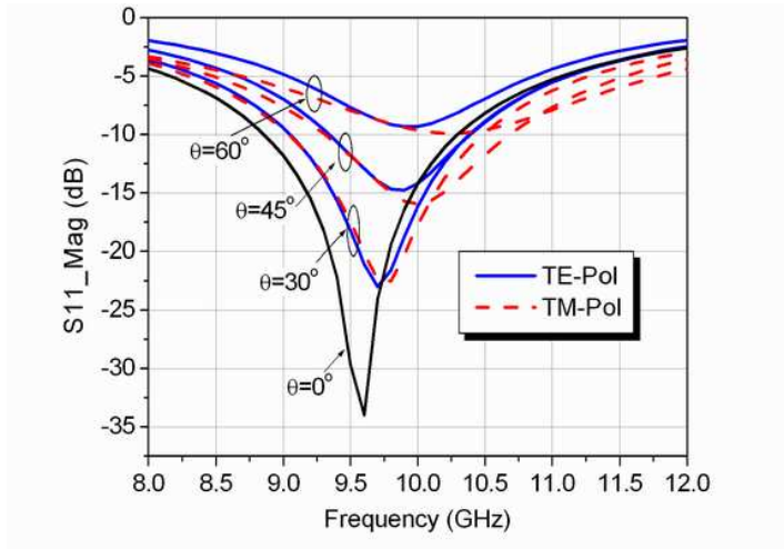
Figure 11. Reflection coefficients characteristics when TE and TM polarized plane wave oblique incidence on JCS absorbing structure.
