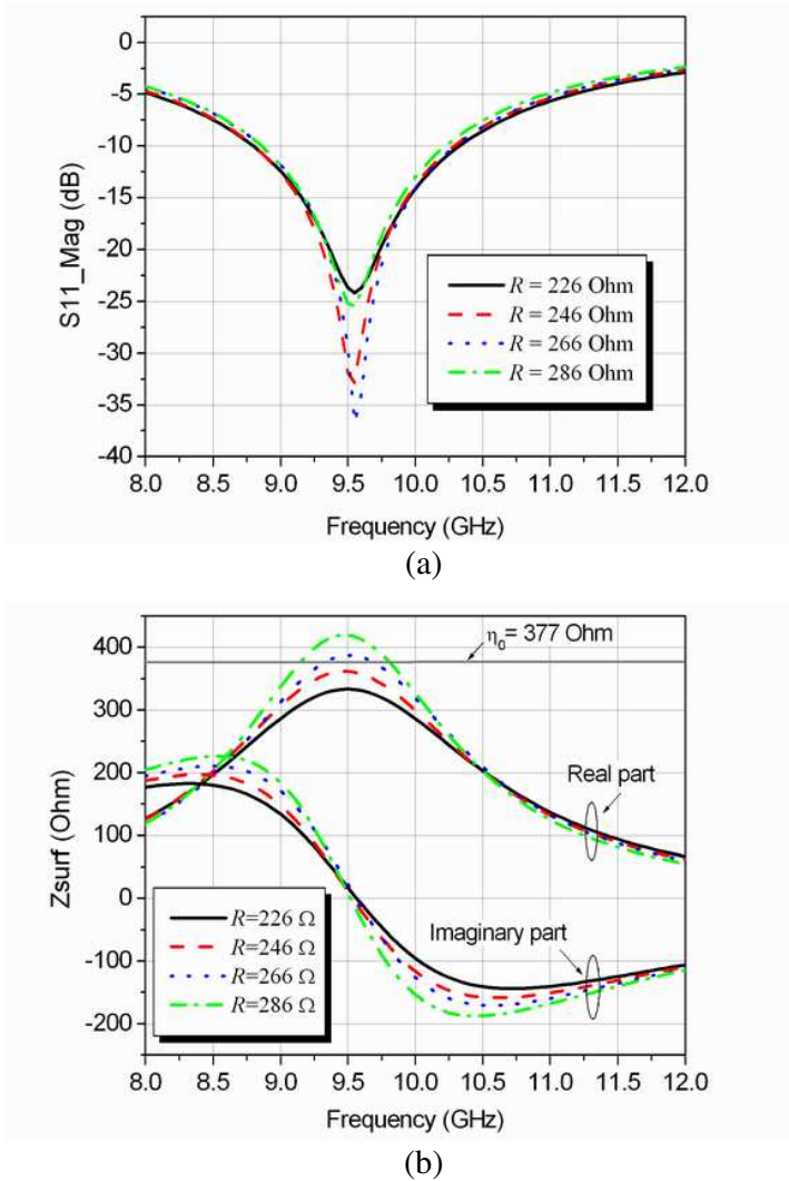
Figure 8. (a) Reflection coefficient curve of variation with load resistance R . (b) Effective surface impedance characteristics of variation with load resistance R .
