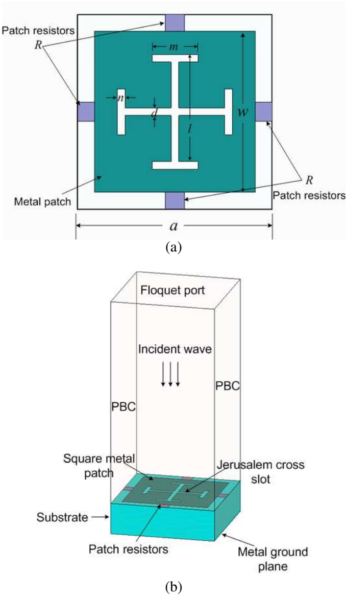
Figure 2. (a) Geometry of JCS. (b) Simulation model of infinite periodic element of absorbing structure using JCS in which the periodic boundary conditions (PBC) are put around the JCS cell.
