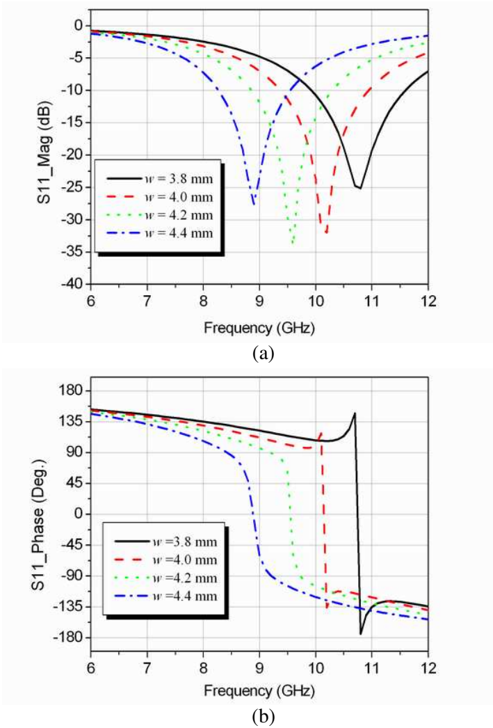
Figure 7. Reflection coefficient variation with the width of square metal patch w .
