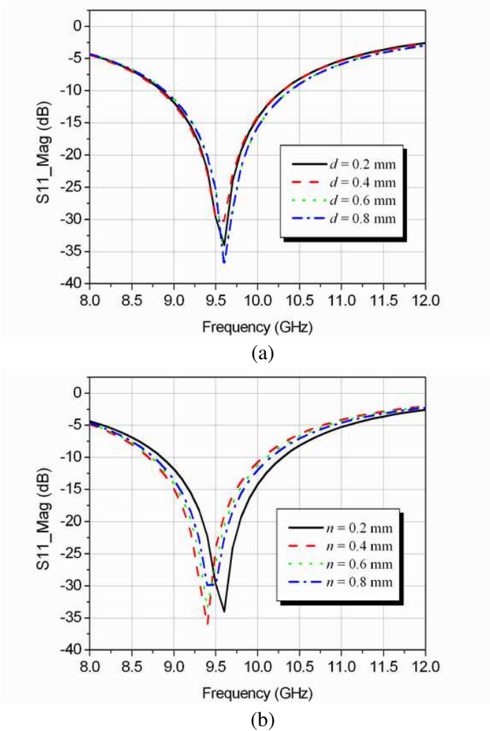
Figure 6. Reflection coefficient variation with JCS width d and n .
