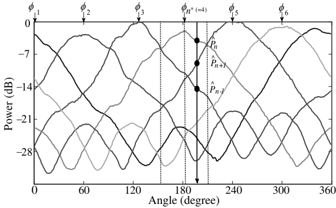
Figure 8. Measured directive beam pattern.
