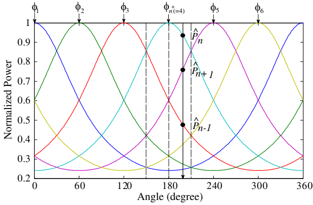
Figure 2. Six directive beam patterns.
