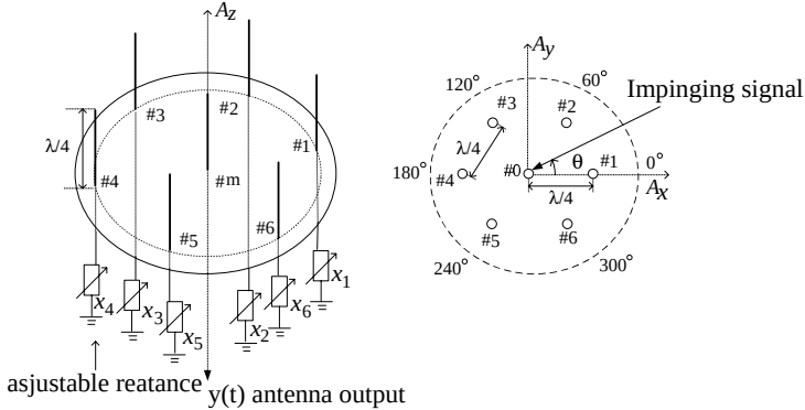
Figure 1. (a) Diagram of ESPAR antenna, (b) 7-element ESPAR antenna.
