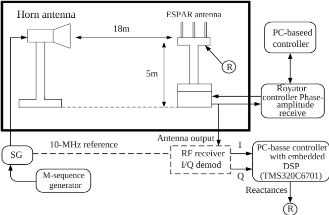
Figure 10. Experimental environment and measurement system setup.
