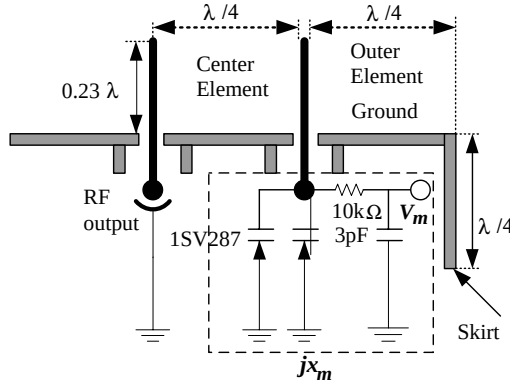
Figure 7. Cross-section of ESPAR antenna circuit.
