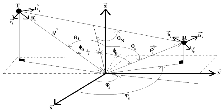
Figure 1. Radar configuration.
