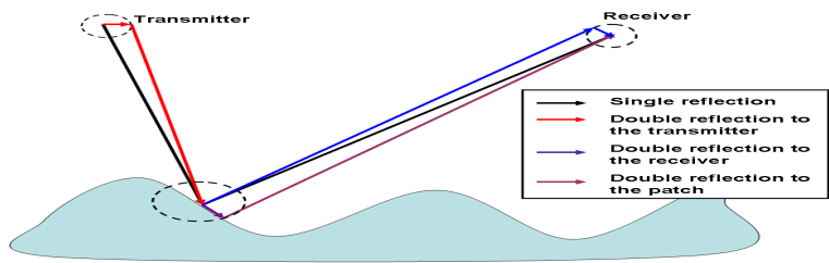
Figure 2. Gill's model.
