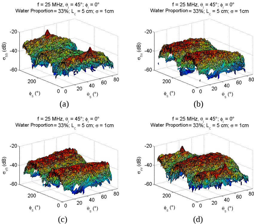
Figure 25. Evolution of the RCS in relation to the receiver position estimated by SSA. (a) \sigma_{hh} . (b) \sigma_{hv} . (c) \sigma_{vh} . (d) \sigma_{vv} .
