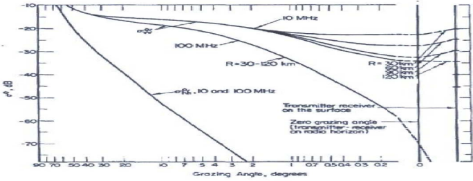
Figure 17. Barrick's RCS [22].
