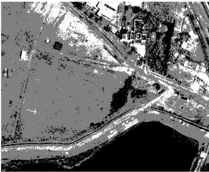
Figure 3. 3-level thresholding.
