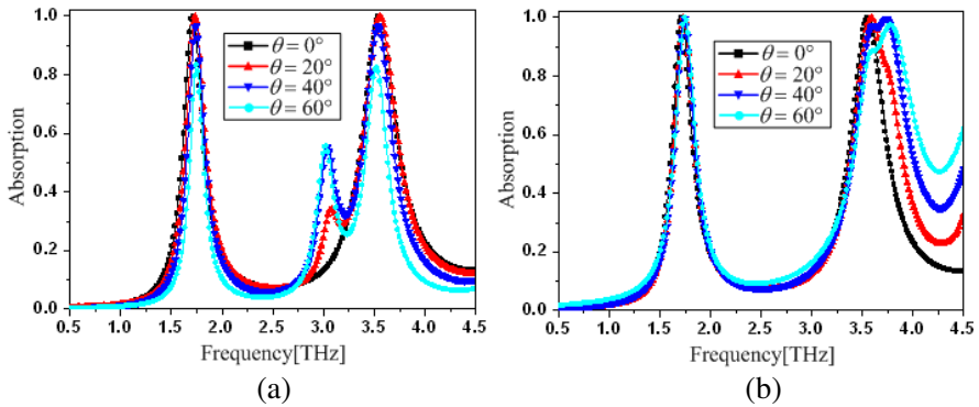
Figure 8. Absorption curves for different oblique incidences at \phi = 0 : (a) TE modes and (b) TM modes.
