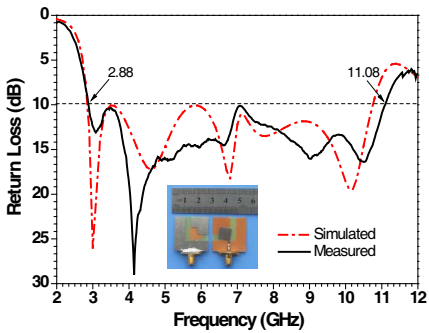
Figure 2. Simulated and measured return losses of the proposed antenna with L = 9\text{ mm} , W = 9\text{ mm} , \alpha = 7.75^\circ , and l = 5\text{ mm} .
