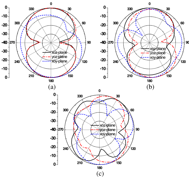
Figure 6. Radiation far-field patterns of the proposed step-slot antenna operation at (a) 3.5 GHz, (b) 6 GHz, and (c) 9 GHz, respectively.
