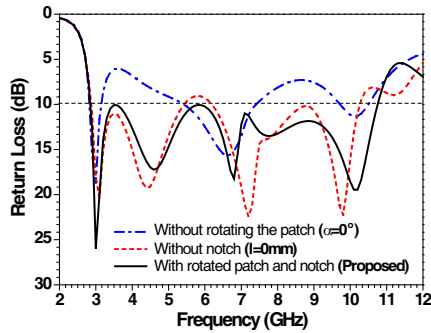
Figure 3. Simulated return losses of the proposed antenna with and without rotated patch and notch.
