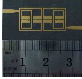
Figure 6. A photograph of the proposed filter.
