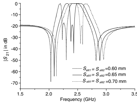
Figure 5. Simulated |S_{21}| of the proposed filter with varied s_{slit1} and s_{slit2} .
