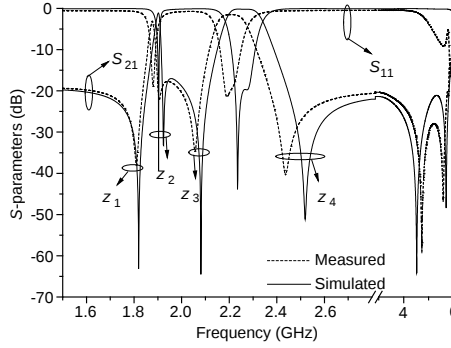
Figure 7. Simulated and measured S -parameters of the proposed filter.
