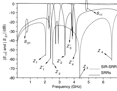
Figure 3. Comparison of the simulated S -parameters of the BPF with SIR-SRR and the conventional SRRs.
