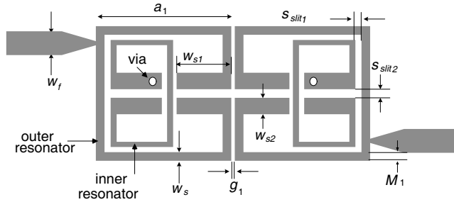
Figure 4. Configuration of proposed filter.
