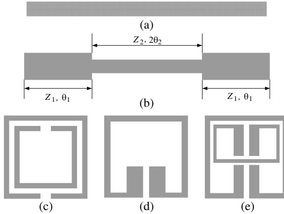
Figure 1. In each row of this figure represents the top view of a resonant magnetic particle. (a) UIR. (b) SIR. (c) SRRs. (d) SIR-SRR. (e) SIR-SRRs.
