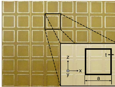
Figure 1. A slide of the metamaterial sample composed of periodic square closed rings.
