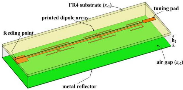
Figure 2. The proposed sleeve dipole array antenna structure.
