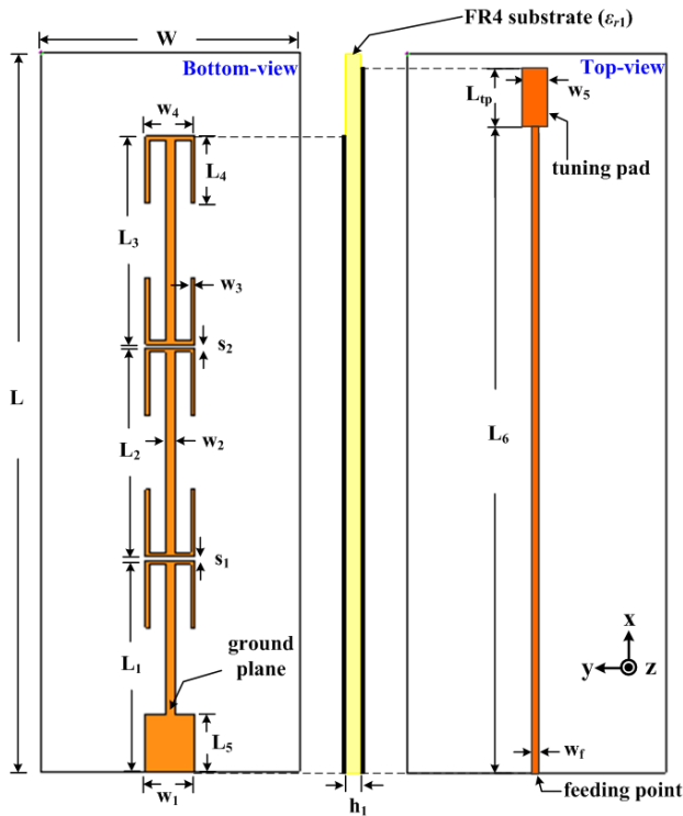
Figure 1. Dimensions of the proposed sleeve dipole array antenna.
