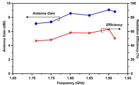
Figure 6. Measured results of antenna gain and radiation efficiency.
