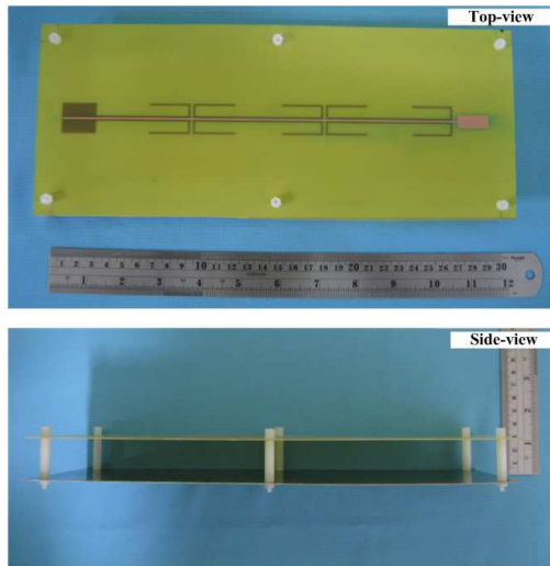
Figure 8. Photography of the planar sleeve dipole array antenna.
