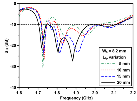
Figure 4. Variations of the simulated S_{11} of different L_{tp} values.
