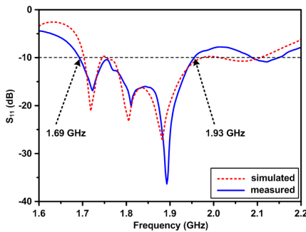
Figure 3. Measured and simulated results of S_{11} .
