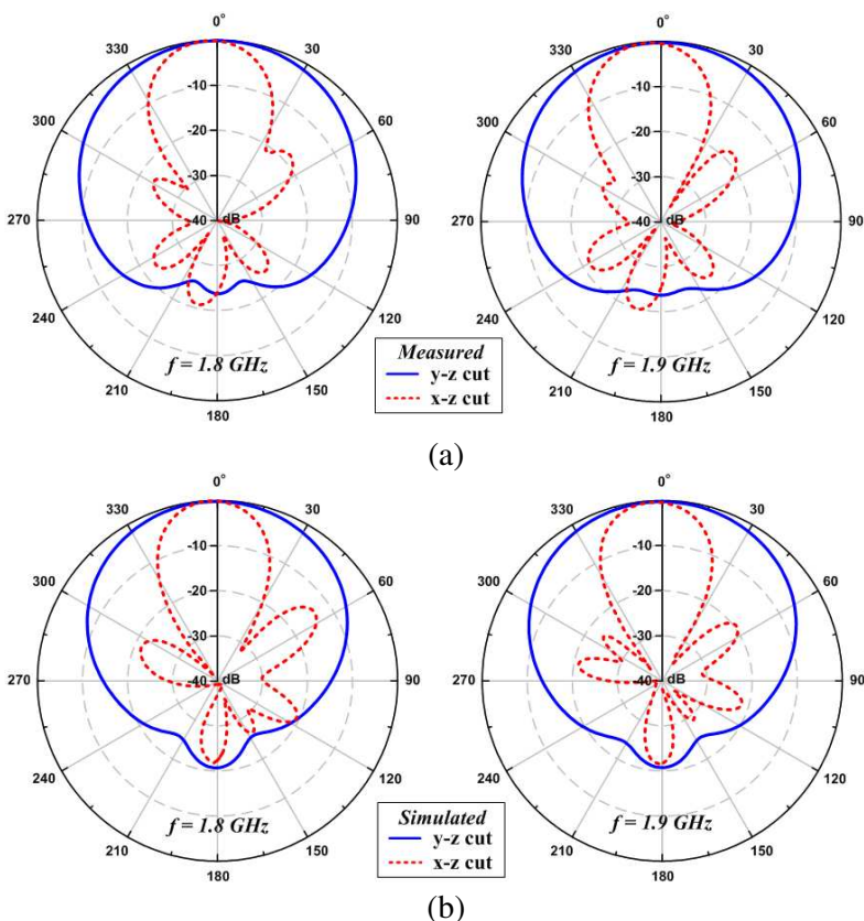
Figure 5. Measured Radiation patterns of the proposed antenna. (a) Measured. (b) Simulated.
