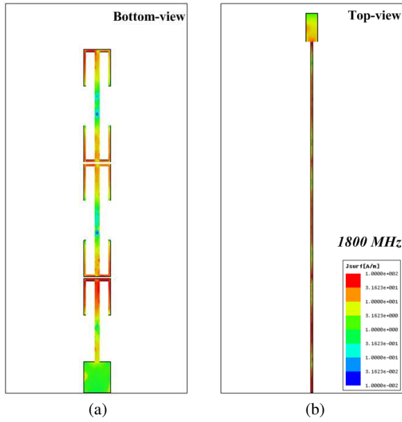
Figure 7. Current distribution.
