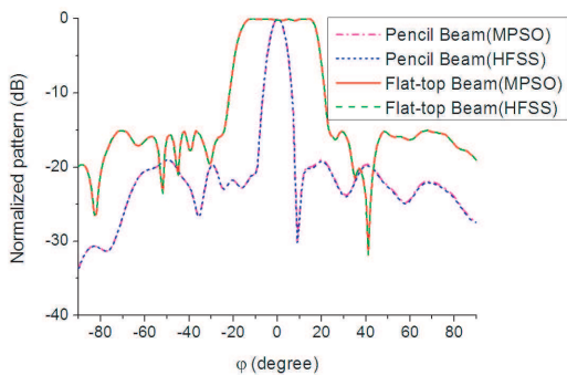
Figure 8. A comparison between the optimized array pattern by MPSO and the exact pattern simulated via HFSS.
