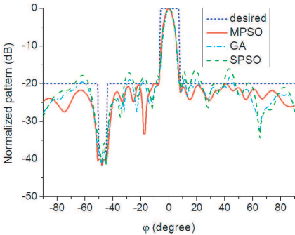
Figure 5. Radiation pattern for the null-shaped beam synthesis.
