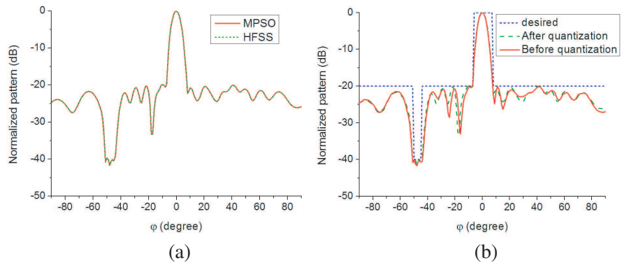
Figure 6. (a) A comparison between the optimized array pattern by MPSO and the exact pattern simulated via HFSS and (b) a comparison between the patterns with amplitudes and phases before and after quantization.
