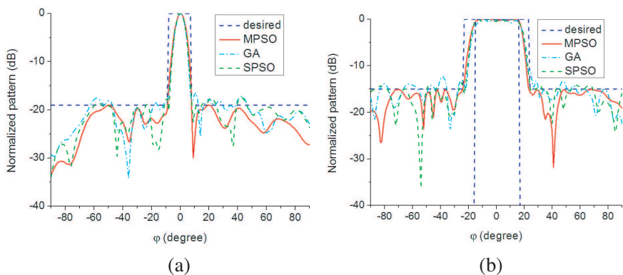
Figure 7. Radiation patterns for the dual-beam array, (a) pencil beam and (b) flat-topped beam.
