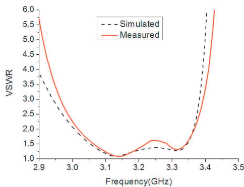
Figure 3. Simulated and measured VSWR for the antenna.
