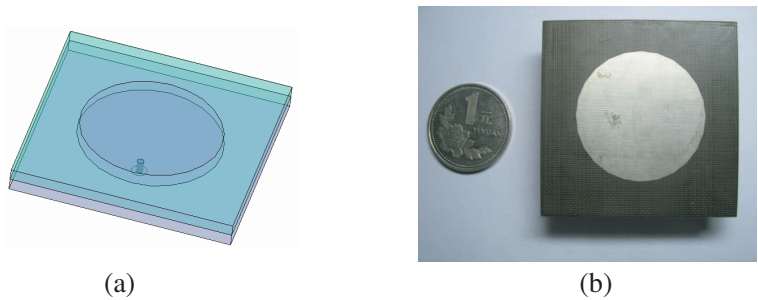
Figure 2. (a) Geometry of the coaxial-fed, stacked patch antenna, and (b) photograph of the fabricated antenna.
