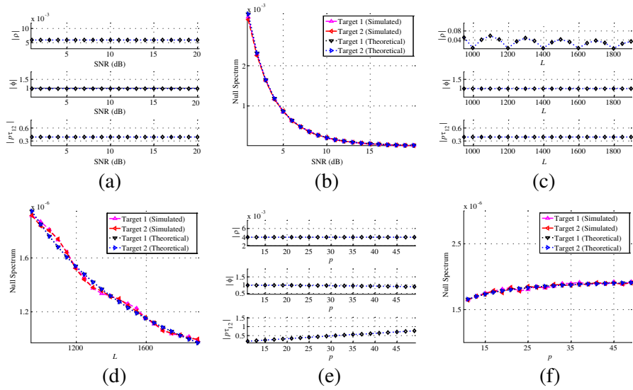
Figure 6. The curves of the null spectrum relative to (a)(b) SNR ( p = 25 , L = 1000 ), (c)(d) L ( p = 25 , SNR = 30 dB) and (e)(f) p ( L = 1000 , SNR = 30 dB) when \phi \neq 0 .
