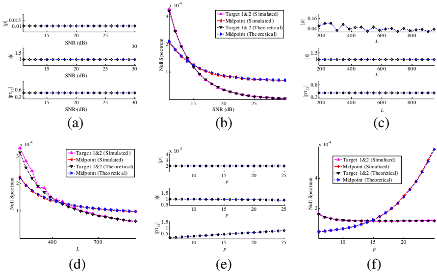
Figure 7. The curves of the resolution threshold relative to (a)(b) SNR ( p = 15 , L = 500 ), (c)(d) L ( p = 15 , SNR = 20 dB) and (e)(f) p ( L = 500 , SNR = 15 dB) when \phi \neq 0 .
