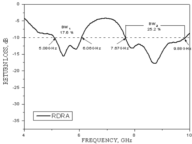
Figure 2. Plot of return loss (RL) versus frequency (GHz) response of RDRA ( h_{dr} = 6 mm).
