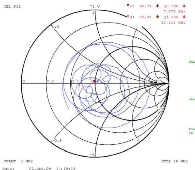
Figure 8. Measured input impedance characteristics on Smith chart.
