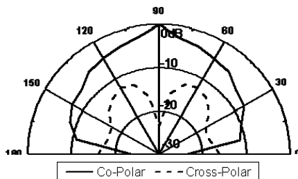
Figure 7. Radiation pattern of MPDRA at 7.07 GHz.
