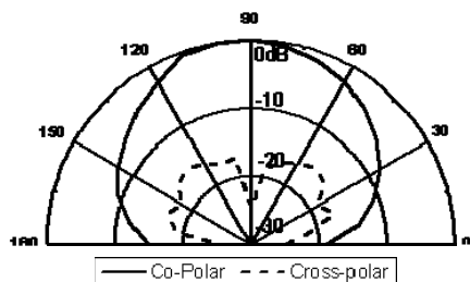
Figure 6. Radiation pattern of MPDRA at 3.57 GHz.
