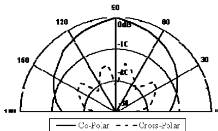
Figure 5. Radiation pattern of RDRA at 8.72 GHz.
