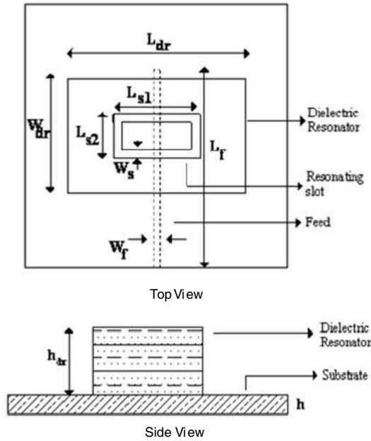
(a) Geometry of RDRA
