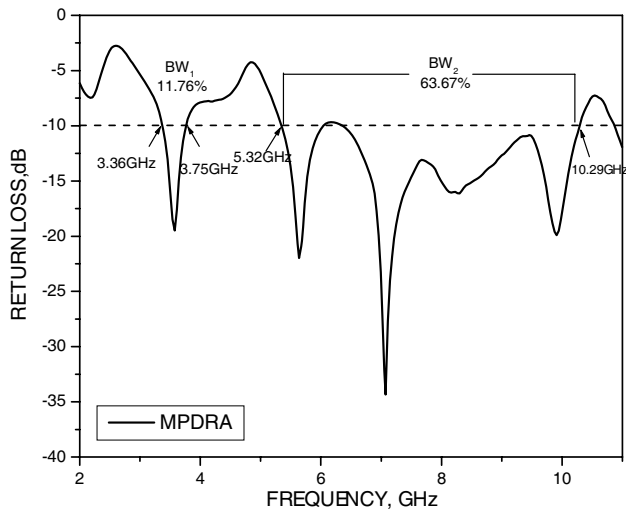
Figure 3. Plot of return loss (RL) versus frequency (GHz) response of MPDRA ( h_{dr} = 6 mm).
