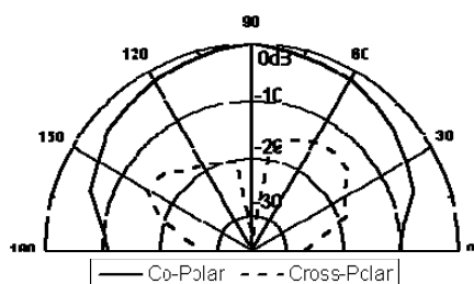
Figure 4. Radiation pattern of RDRA at 5.43 GHz.
