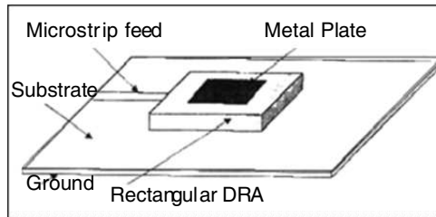
(b) Geometry of MPDRA
