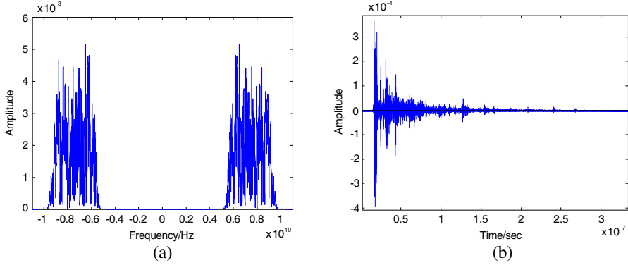
Figure 3. (a) Measured transfer function in [6 9] GHz without antenna calibration. Notice that, a conjugate symmetric spectrum has been constructed. (b) The extracted discrete UWB CIR after windowing, antenna calibration and time-domain deconvolution.
