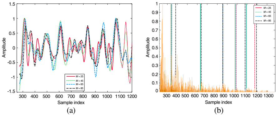
Figure 7. Effects from averaging length M . (a) Wavelet coefficients under different M . (b) Cluster identification results under different M . Notice that, in this experiment, the scale value \alpha is set to 51.
