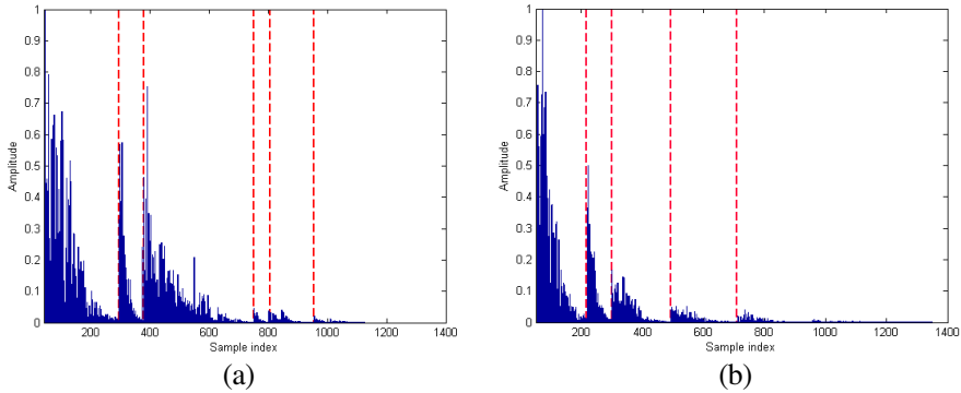
Figure 9. Cluster identification realizations for the IEEE 802.15.4a channel modeling. The cluster arrival interval in CIR generation program is defined to 22.32 ns, and the estimated value based on 50 independent realizations is about 24 ns. (a) The LOS case; and (b) the NLOS case. Notice that, for the NLOS case, the first and third cluster may not exactly follow an exponential decay rule.
