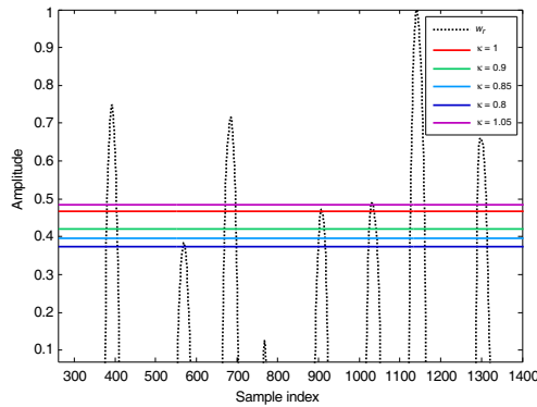
Figure 8. Disturbance analysis of the suggested threshold scheme.
