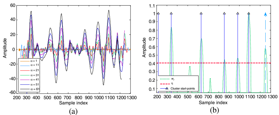
Figure 6. (a) Wavelet coefficients of the MAR signal under different scale values. (b) Wavelet based cluster identification.
