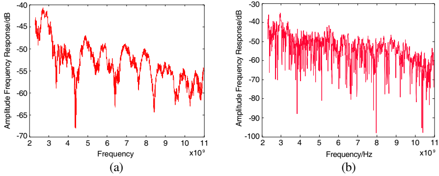
Figure 2. (a) Amplitude frequency response A(f) of the omnidirectional UWB antennas. (b) The amplitude of measured UWB channel transfer function, i.e., S(f) .
