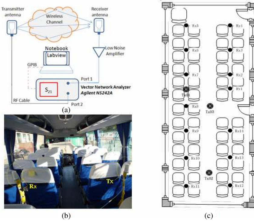
Figure 1. (a) Typical setup for the frequency-domain measurement. (b) The testing scene in vehicle cabin. (c) The topology of vehicle cabin and measurement antennas deployment.
