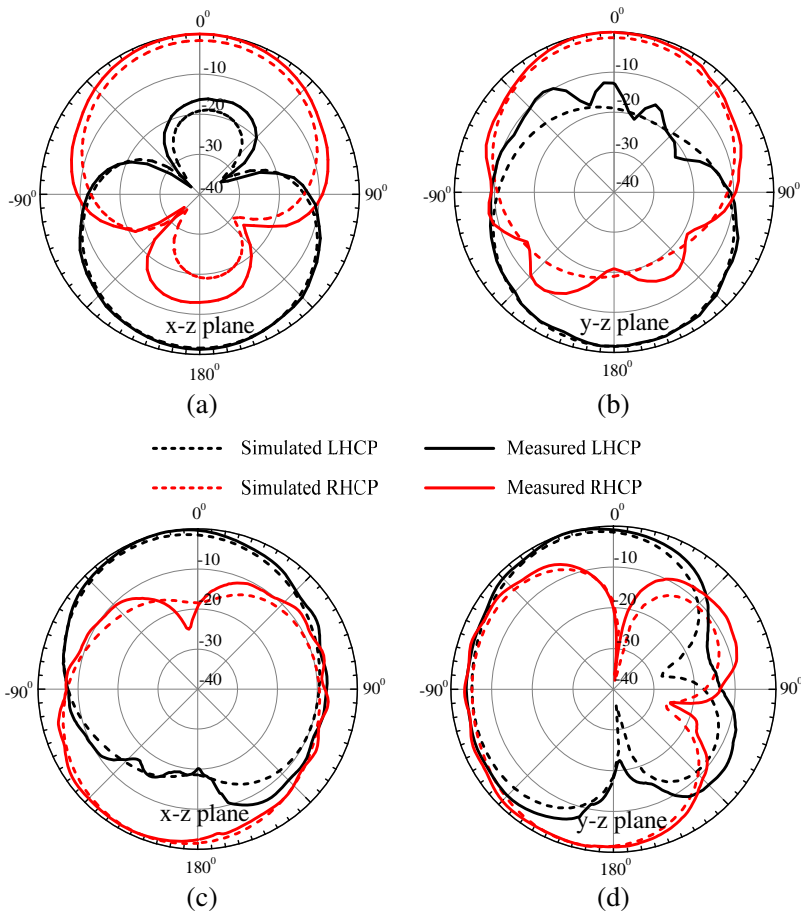
Figure 7. Radiation patterns: (a) x-z plane, (b) y-z plane at 1.57 GHz, (c) x-z plane, (d) y-z plane at 2.46 GHz.
