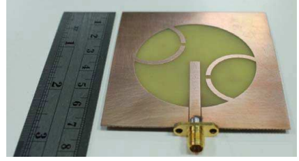
Figure 9. Photograph of proposed antenna.
