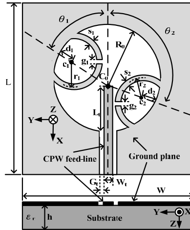
Figure 1. Configuration of the proposed CPW-fed slot antenna.
