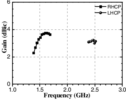
Figure 8. Measured antenna gains.
