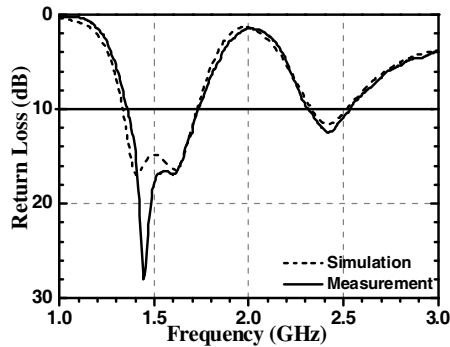
Figure 3. Return loss spectrums of the proposed antenna.
