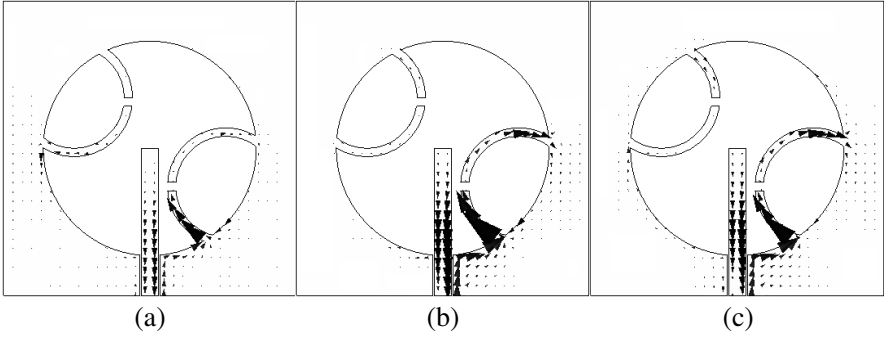
Figure 6. Simulated vector current distributions at 2.46 GHz, (a) 0 degree, (b) 45 degree, (c) 90 degree.
