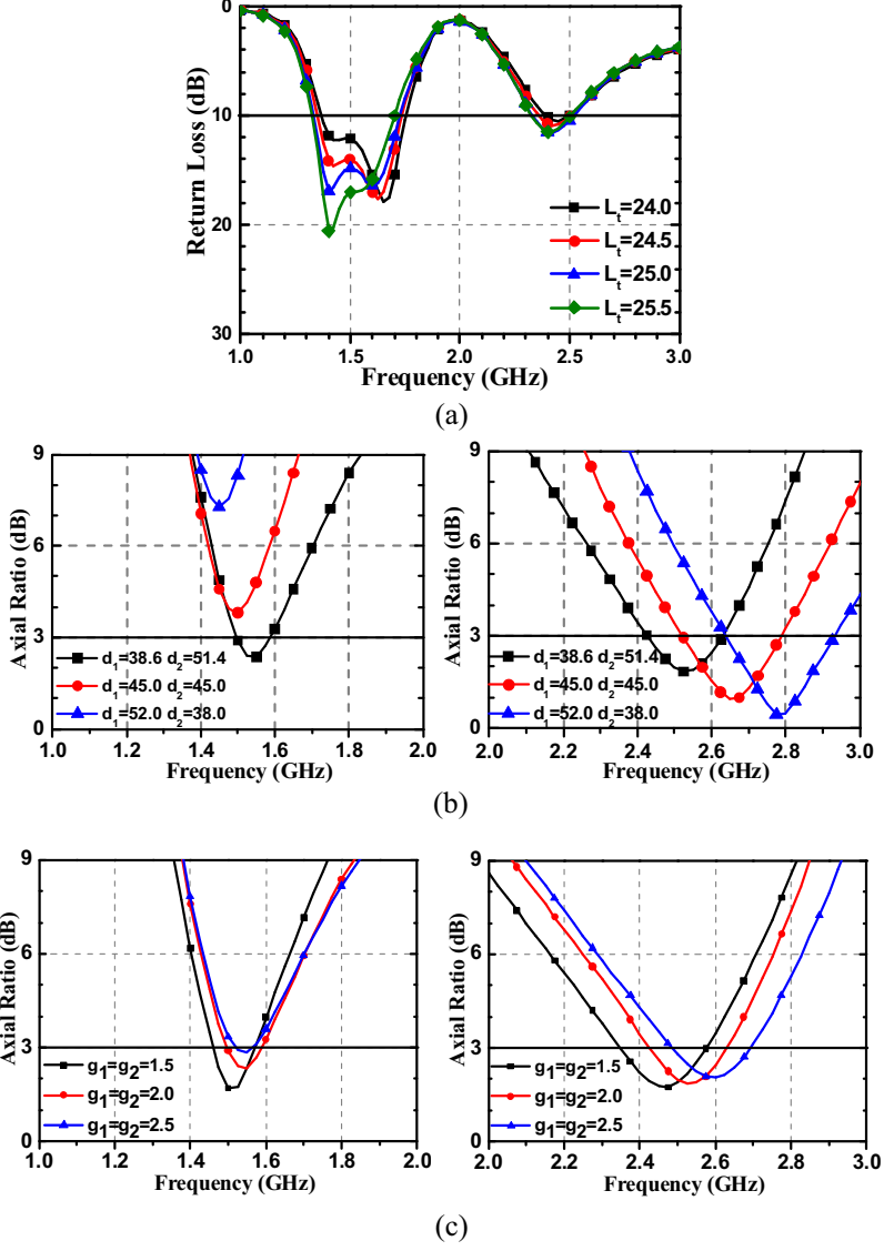
Figure 2. Characteristics of the parameter variations. (a) Variation of feed strip length. (b) Variation of radius of two opened-ground rings. (c) Variation of gaps of two opened-ground rings.
