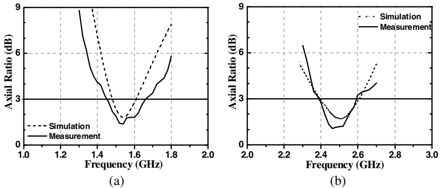
Figure 4. Axial ratio spectrums (a) 1.57 GHz, (b) 2.46 GHz.
