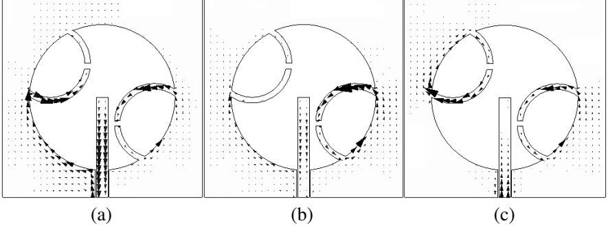
Figure 5. Simulated vector current distributions at 1.57 GHz, (a) 45 degree, (b) 90 degree, (c) 135 degree.
