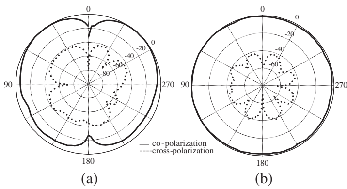
Figure 9. Measured antenna radiation patterns at 4 GHz: (a) E -plane; (b) H -plane.
