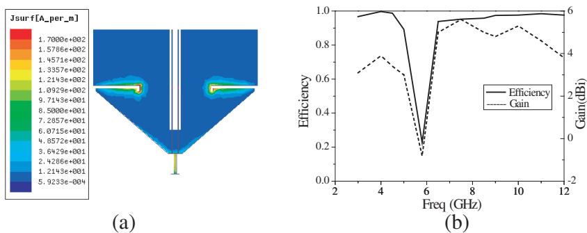
Figure 8. (a) Simulated current distribution of the propose antenna at 5.8 GHz and (b) gain and efficiency of the propose antenna.
