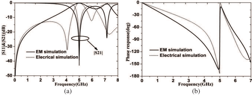
Figure 2. S -parameters of the CELC-loaded SN MTM cell obtained from full-wave EM simulation and electrical simulation. (a) Magnitude response, (b) transmission phase response. The physical parameters of the CELC-loaded cell are: w_s = 2.2 mm, g = 0.2 mm, L = 7 mm, h = 4.6 mm, and dimension of the entire cell is 9 mm. Extracted lumped-element parameters are: L_s = 1.44 nH, C_s = 0.12 pF, L_g = 8.44 nH, L_p = 3.57 nH, C_p = 0.13 pF and R = 12.3 \Omega .
