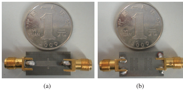
Figure 7. Fabricated prototype of the designed BSF using two cascaded H-CELC cells. (a) Top view and (b) bottom view. The width and height of open stub in the center of conductor strip are 0.8 mm and 5.4 mm, the distance (periodicity) between the two cells is 7 mm.
