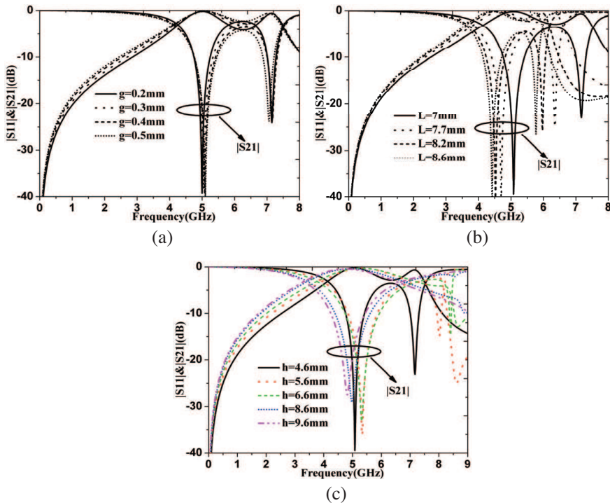
Figure 4. S -parameters of the CELC-loaded SN MTM cell with various geometrical parameters. (a) Various g ( L = 7 mm, h = 4.6 mm), (b) various L ( g = 0.4 mm, h = 4.6 mm), (c) various h ( g = 0.4 mm, L = 7 mm).
