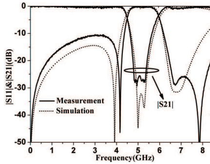
Figure 8. Simulated and measured S -parameters of the proposed BSF.
