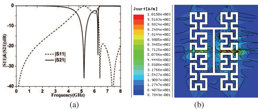
Figure 6. Simulated results of the designed SN MTM cell based on H-CELC. (a) S -parameters obtained from Ansoft Designer. (b) Current distribution from Ansoft HFSS.
