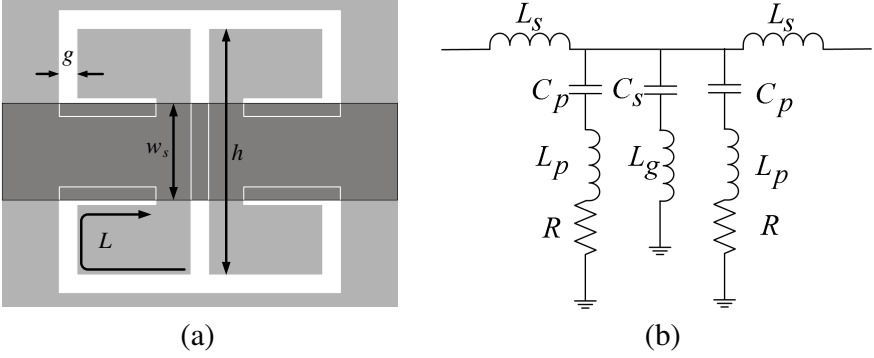
Figure 1. (a) Topology and (b) corresponding lumped-element equivalent circuit model of the SN MTM cell. The CELC (depicted in white) is etched in the ground (depicted in light grey) underneath the conductor strip (depicted in dark grey).
