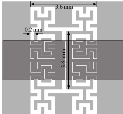
Figure 5. Layout of the proposed SN MTM cell based on H-CELC.
