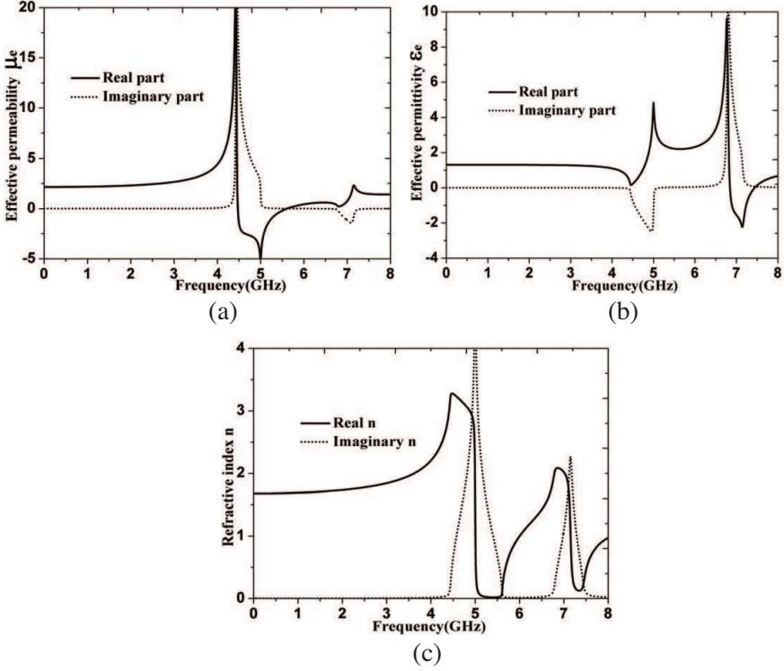
Figure 3. Constitutive EM parameters of CELC-loaded SN MTM cell. (a) Effective permeability, (b) effective permittivity and (c) refractive index.
