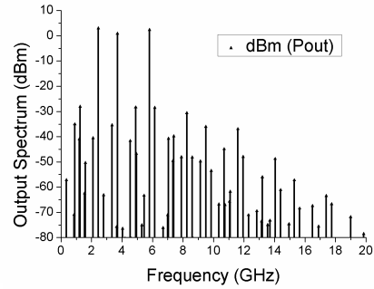
Figure 12. Output spectrum with simultaneous 3-band signal input.
