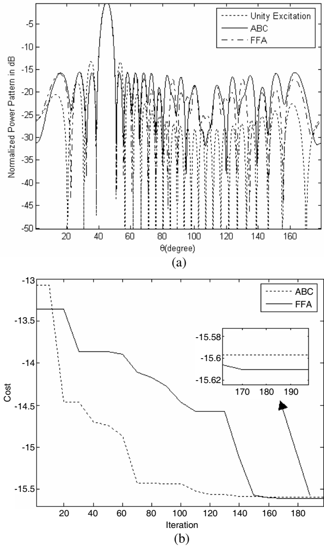
Figure 6. (a) Normalize Power Patterns steered at 45^\circ with 26 elements array using FFA and ABC. (b) Convergence curves of the scanned array steered at 45^\circ with 26 elements using FFA and ABC.
