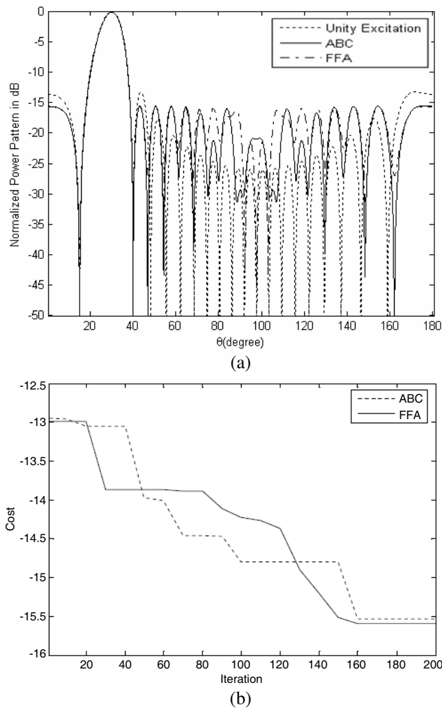
Figure 5. (a) Normalized Power Patterns steered at 30^\circ with 20 elements array using FFA and ABC. (b) Convergence curves of the scanned array steered at 30^\circ with 20 elements using FFA and ABC.
