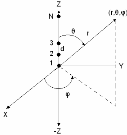
Figure 1. Linear array of isotropic sources along z -axis.
