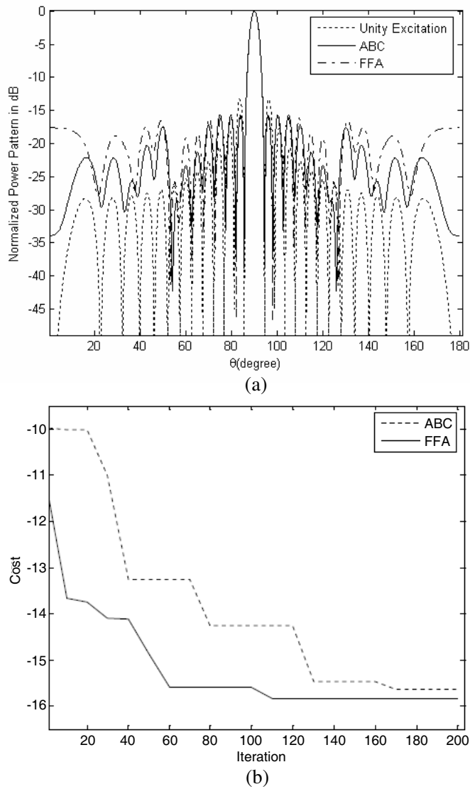
Figure 3. (a) Normalized Power Patterns with 26 elements broadside array using FFA and ABC. (b) Convergence curves of 26 elements broadside array using FFA and ABC.
