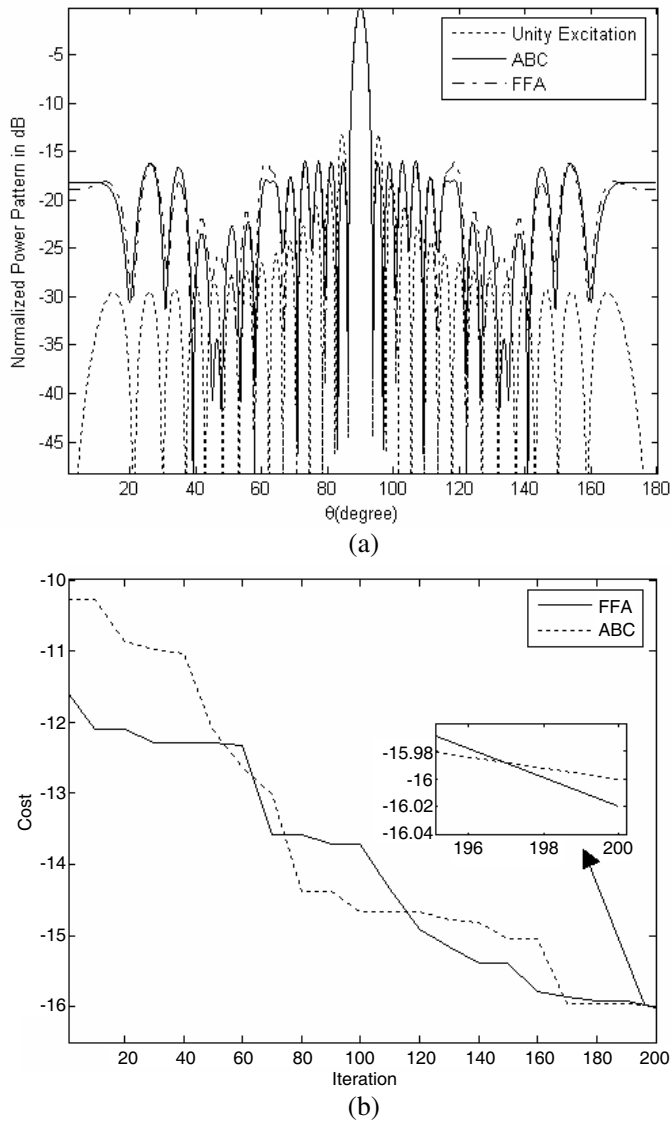
Figure 4. (a) Normalized Power Patterns with 30 elements broadside array using FFA and ABC. (b) Convergence curves of 30 elements broadside array using FFA and ABC.
