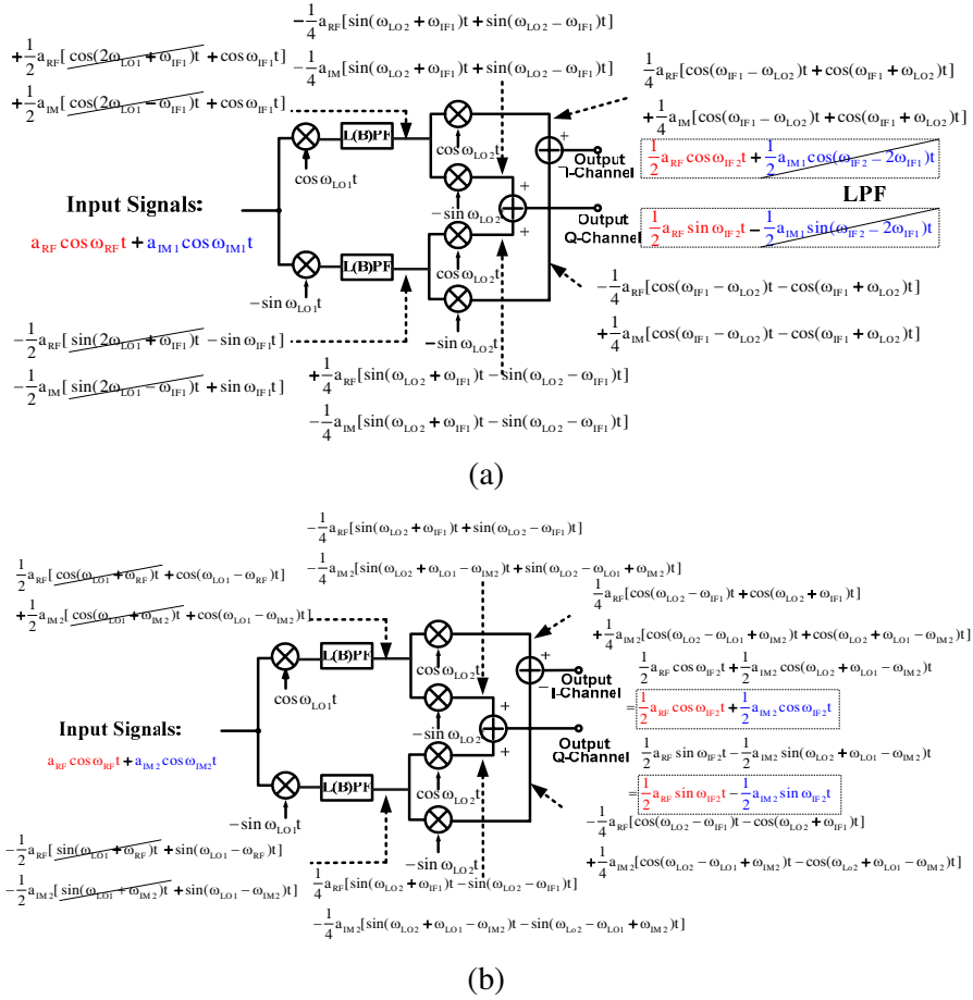
Figure 3. Block diagram of the Weaver architecture, (a) when input signals are desired RF signal and first image signal, (b) when input signals are desired RF signal and second image signal.
