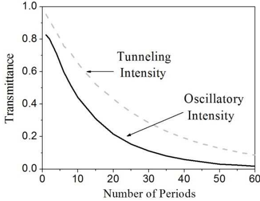
Figure 6. Peaks of transmittance through samples of finite number of periods. The waves are TE, the angle of incidence from air is 30^\circ and \gamma = 0.01\omega_0 . The transmitting medium is also air. The curves in this figure correspond to the maximum of transmission along the oscillatory and tunneling regions.
