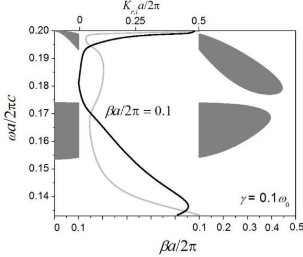
Figure 4. The same as Figure 3 but considering absorption mechanisms. The projected bands correspond to regions — over the complete plane of the figure — where the imaginary Bloch wave vector satisfies K_i a/2\pi \leq 0.07 . To visualize the complex curve of dispersion at \beta a/2\pi = 0.1 we use the same upper scale for K_r and K_i .
