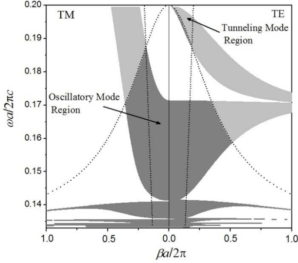
Figure 2. The projected TM and TE photonic bands. The Gaussian-type dotted curve is the metamaterial light-curve. The dotted right lines define the light-cone. For any \beta value, the borders of the projected bands correspond to the borders of the Brillouin zone. The arrows indicate the two regions inside the light-cone of interest in this work. The darker regions for both TE and TM polarizations correspond to oscillatory modes; the light gray region for TE polarization inside the light-cone contains the tunneling modes.
