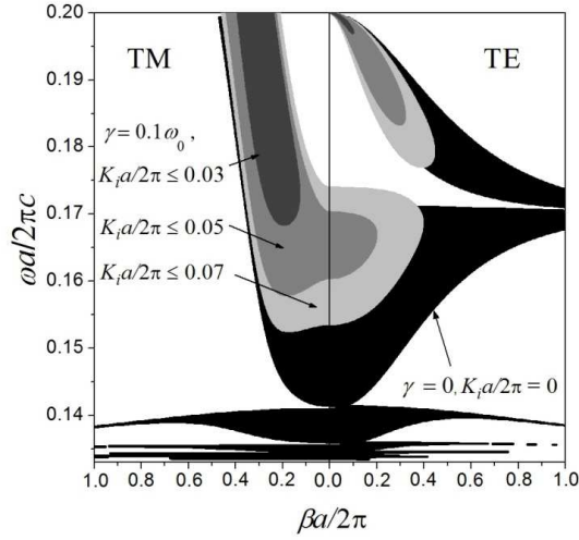
Figure 5. Complex projected photonic bands that show the effect of the absorption on the field penetration into the superlattice. The fields decay exponentially due to the imaginary Bloch wave vector component. As smaller is this component, larger is the field penetration.
