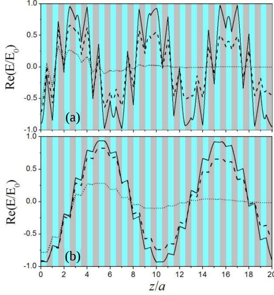
Figure 7. TE field distribution in a sample of 20 bilayers. The wave is incident from air with angle of incidence \theta_i = 30^\circ . Solid line, dashed line and dotted line correspond to absorption parameters \gamma = 0 , \gamma = 0.01\omega_0 and \gamma = 0.1\omega_0 , respectively. (a) Oscillatory mode: \omega a/2\pi c = 0.1607 and \beta a/2\pi = 0.08 , (b) Tunneling mode: \omega a/2\pi c = 0.1962 and \beta a/2\pi = 0.098 .
