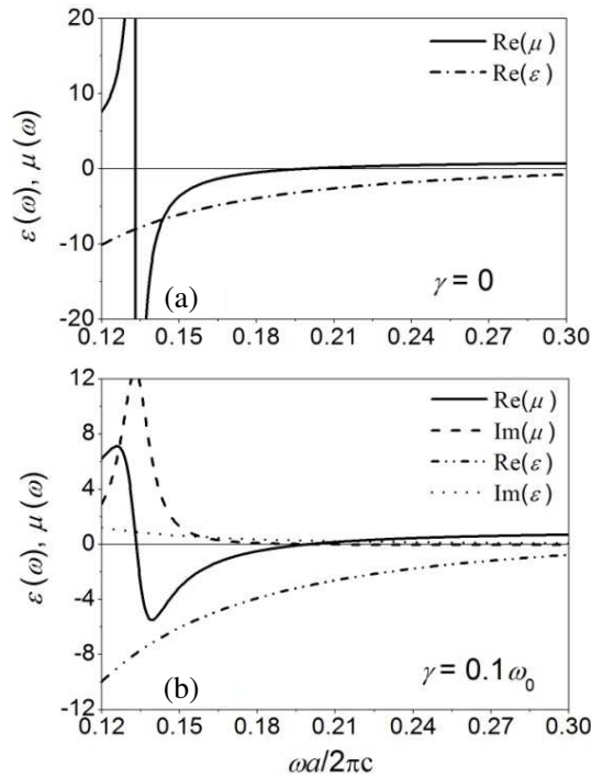
Figure 1. The frequency-dispersive permittivity \varepsilon(\omega) and permeability \mu(\omega) functions. With finite loss parameter \gamma both functions become complex: (a) \gamma = 0 and (b) \gamma = 0.1\omega_0 . The frequency region in which both \text{Re}(\varepsilon) and \text{Re}(\mu) are negative is the metamaterial regime.
