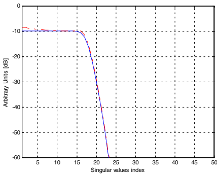
Figure 9. Comparison between the absolute singular values of the two operators (blue line: magnetic source; red dashed line: electric source) in the case X_1 = 10\lambda and z_1 = 20\lambda .
