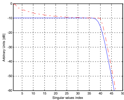
Figure 6. Comparison between the absolute singular values of the two operators (blue line: magnetic source; red dashed line: electric source) in the case X_1 = 20\lambda and z_1 = 5\lambda .
