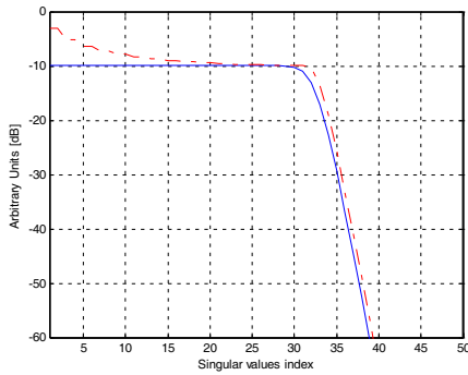
Figure 4. Comparison between the absolute singular values of the two operators (blue line: magnetic source; red dashed line: electric source) in the case X_1 = 10\lambda and z_1 = 5\lambda .
