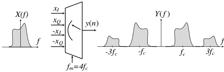
Figure 3. High-speed 4 \times 1 multiplexer working as a frequency up-converter.
