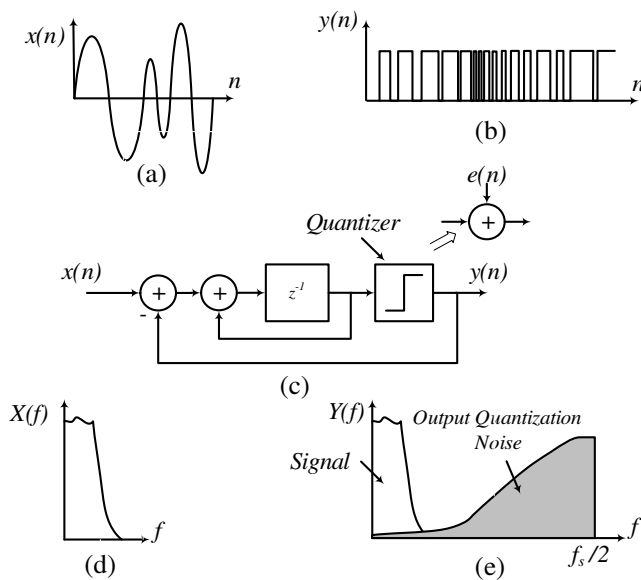
Figure 2. Delta-sigma modulator.
