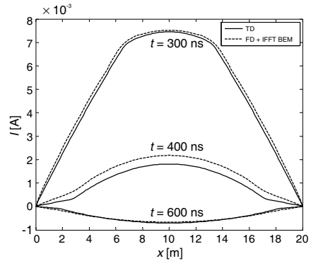
Figure 12. Current along the wire at different time instants, L = 20 m, d = 15 m, \sigma = 1 mS/m.
