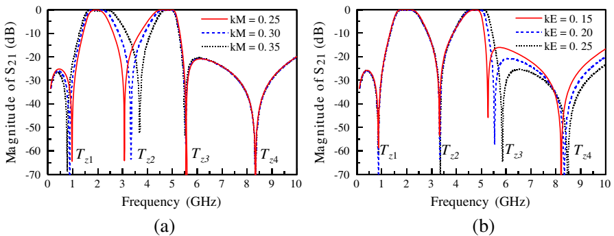
Figure 11. Comparison of the magnitude of S_{21} for the dual-band bandpass filter design with different electrical and magnetic coupling coefficients. (a) Magnitude of S_{21} with varying k_M . (b) Magnitude of S_{21} with varying k_E .
