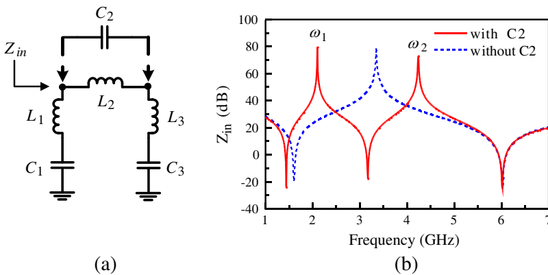
Figure 3. Proposed dual-resonance composite resonator with a parallel capacitor. (a) Equivalent circuit. (b) Magnitude response of input impedance.
