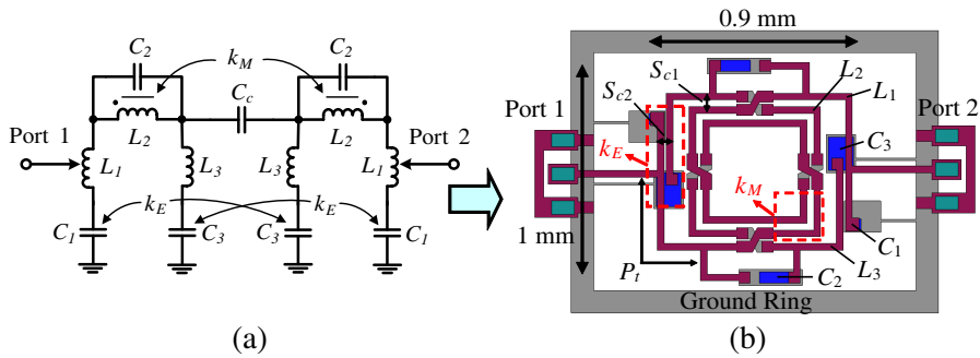
Figure 12. Proposed transformer-coupled dual-band bandpass filter design using glass IPD technology. (a) Equivalent circuit. (b) Corresponding layout structure.
