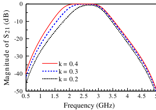
Figure 5. Comparison of operating bandwidth for the dual-mode bandpass filter design with three different coupling coefficients.
