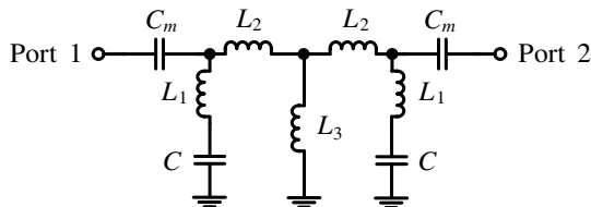
Figure 4. Equivalent circuit of the proposed dual-mode bandpass filter.
