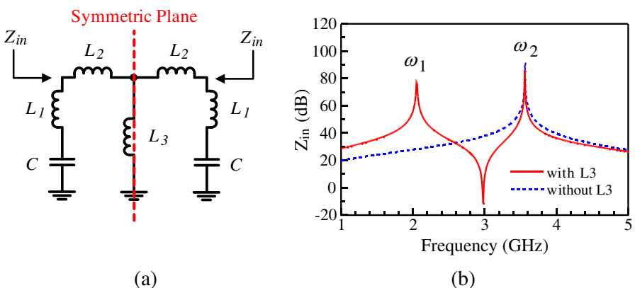
Figure 2. Proposed dual-resonance composite resonator with a grounded inductor. (a) Equivalent circuit. (b) Magnitude response of input impedance.
