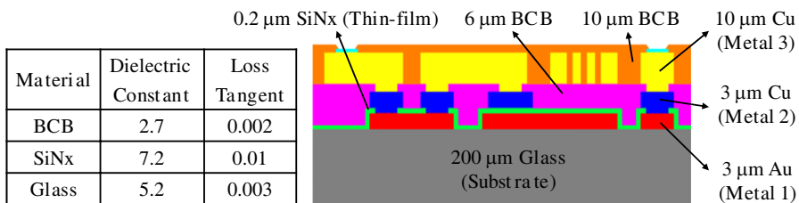
Figure 1. Cross-sectional view and material parameters of the adopted glass IPD technology.
