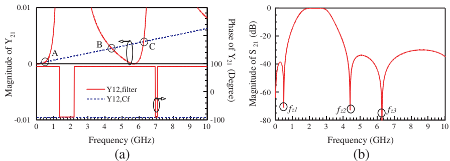
Figure 7. (a) Magnitude and phase responses of the admittance parameters of Y_{12,filter} and Y_{12,Cf} . (b) The magnitude of S_{21} of the proposed dual-mode bandpass filter with a capacitive feedback path.
