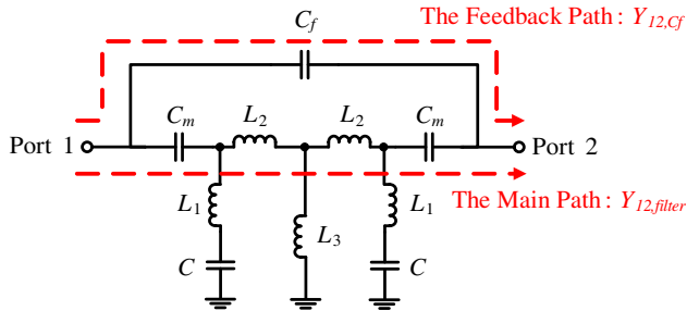
Figure 6. Equivalent circuit of dual-mode bandpass filter with a capacitive feedback path.
