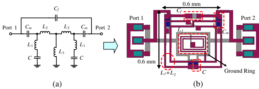
Figure 8. Proposed dual-mode bandpass filter design using glass IPD technology. (a) Equivalent circuit. (b) Corresponding layout structure.
