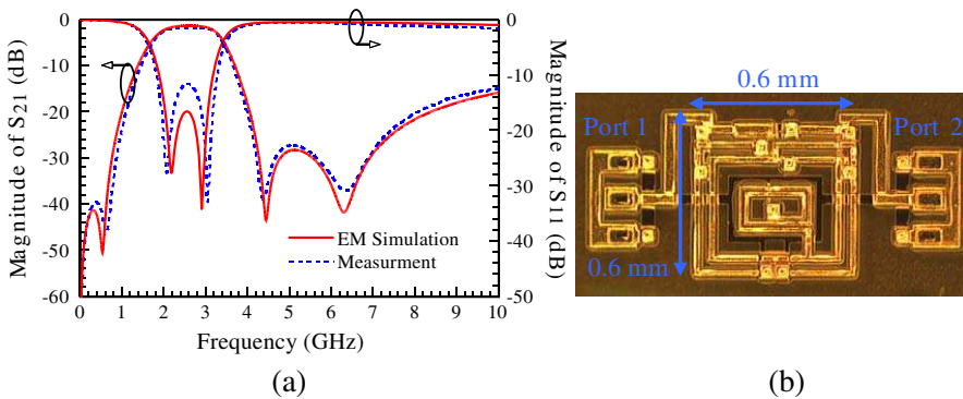
Figure 9. Results and structure of the designed IPD dual-mode bandpass filter. (a) Comparison of the magnitude of S_{21} and S_{11} between EM simulation and measurement. (b) Chip photograph.
