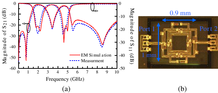
Figure 13. Results and structure of the designed IPD transformer-coupled dual-band bandpass filter. (a) Comparison of the magnitude of S_{21} and S_{11} between EM simulation and measurement. (b) Chip photograph.
