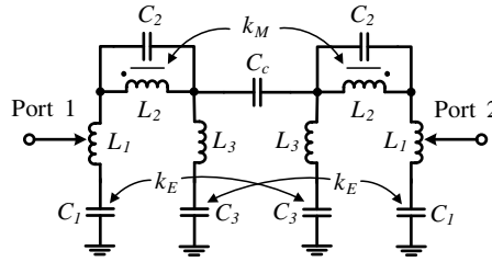
Figure 10. Equivalent circuit of the designed dual-band bandpass filter.
