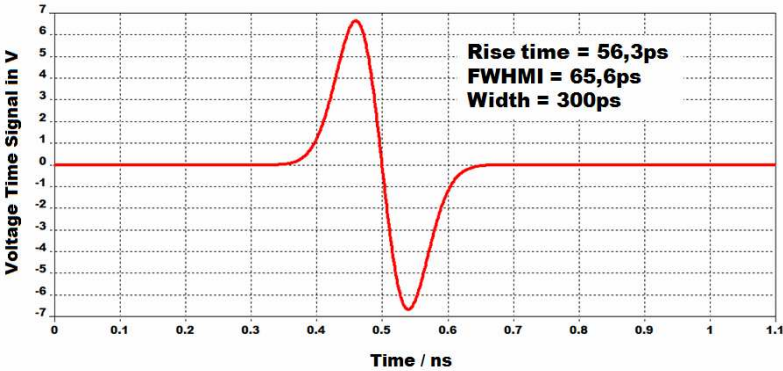
Figure 2. Example of a monocycle pulse shape (duration of 300 ps).
