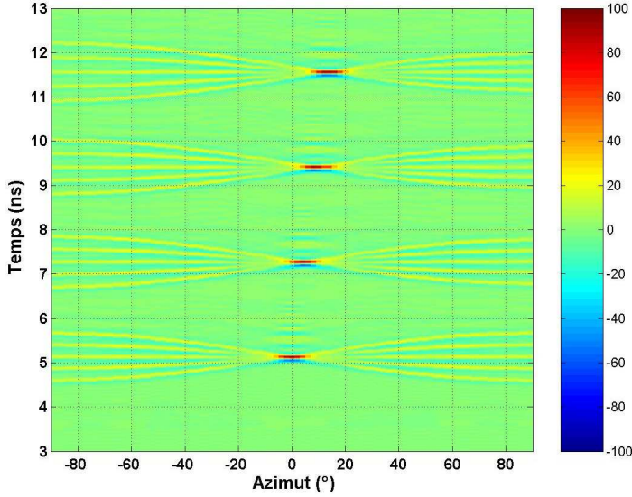
Figure 5. Example of a scanning involved by the system.
