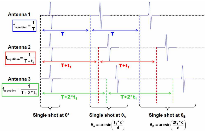
Figure 4. Series of pulses having different repetition frequencies.
