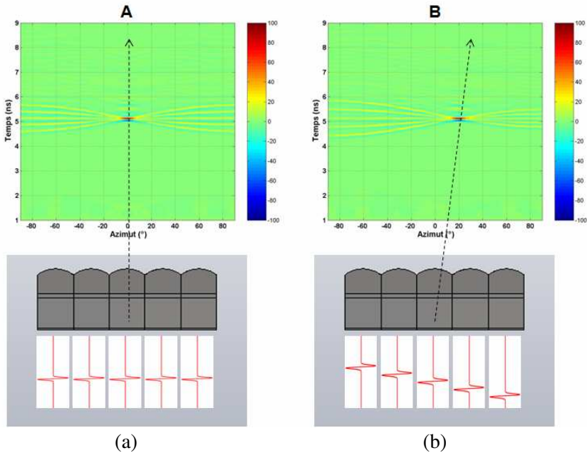
Figure 1. Perfect synchronization of all sources, (a) involving a single shot at the 0^\circ azimuth and application of a delay t_1 between two adjacent sources, (b) involving a single shot at the 20^\circ azimuth.
