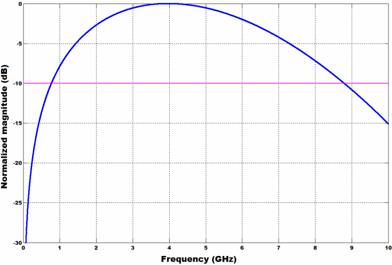
Figure 3. Spectrum of a monocycle pulse, covering a decade of band.
