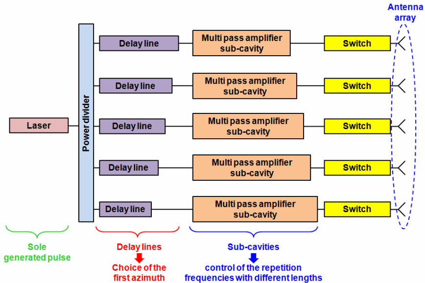
Figure 6. Implementation of the autonomous scan with different sub-cavities.
