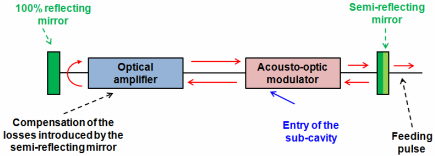
Figure 7. Multipass amplifier constitution.
