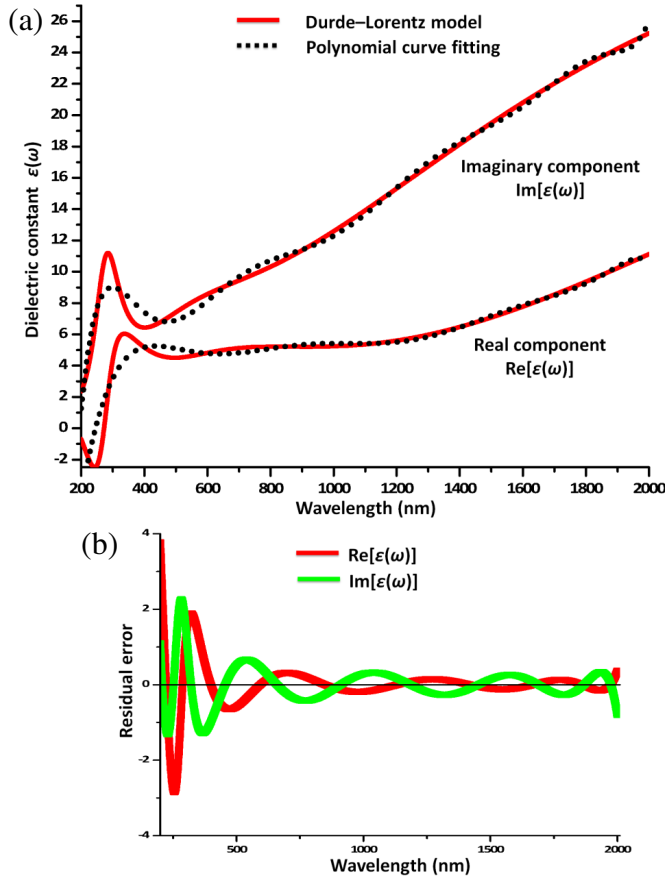
Figure 1. (a) Dielectric function \epsilon_{\perp}(\omega) of carbon nanotubes for light polarized parallel to the nanotube axis. Solid lines represent the Drude-Lorentz model used in reference [16]. The dashed lines represent the polynomial fitted curves. (b) The residual error generated by the curve fitting.
