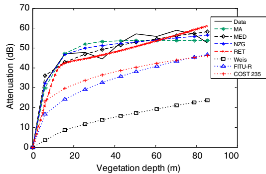
Figure 5. Comparison of attenuation models based on best-fit analysis for measurements at 2.5 GHz in oil palm plantation.
