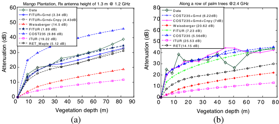
Figure 6. Comparison of vegetation attenuation models at; (a) 1.2 GHz in mango plantation, (b) 2.4 GHz along a row of oil palm trees.
