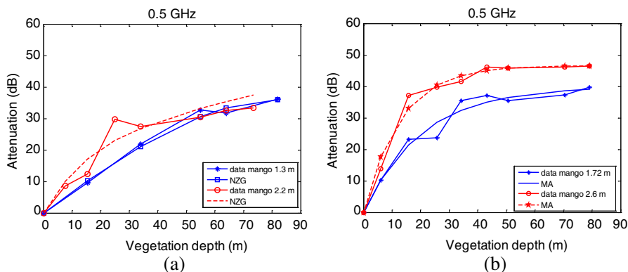
Figure 3. Vegetation attenuation of 500 MHz signal (mango plantation) at (a) location 1 and (b) location 2 for different antenna heights and best-fit model.
