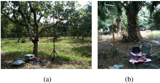
Figure 2. Experimental measurement set-up in (a) mango plantation — transmitter and, (b) oil palm plantation — receiver.
