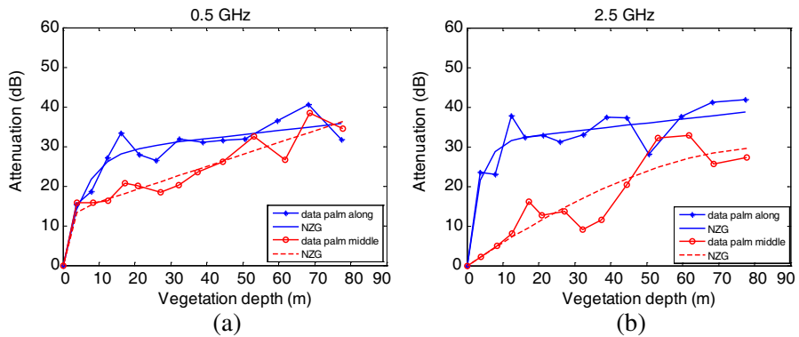
Figure 4. Signal attenuation along a row of palm trees and in-between two rows of palm trees for transmissions at (a) 500 MHz and, (b) 2.5 GHz.
