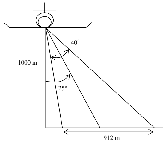
Figure 2. Geometric configuration of the UAVSAR system.
