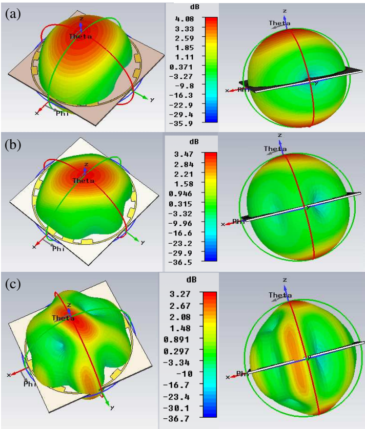
Figure 6. 3D gain calculated by CST Microwave Studio at the frequency of (a) 866.6 MHz, (b) 2.45 GHz, (c) 4 GHz.
