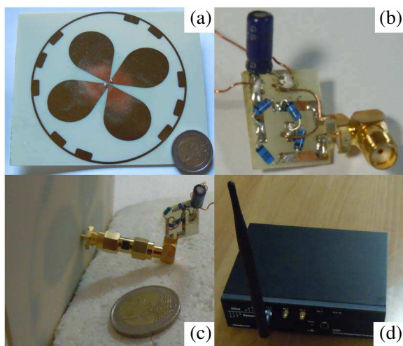
Figure 3. Photographs of the realized rectenna: (a) the antenna, (b) the rectifier, (c) the antenna connected to the rectifier, (d) the USRP adopted to generate the signal incident on the rectenna.
