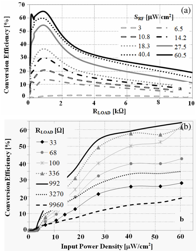
Figure 7. Measurements of \eta_{RFtoDC, rectenna} : RF-to-DC conversion efficiency (a) as function of the load and (b) as function of the input power density.
