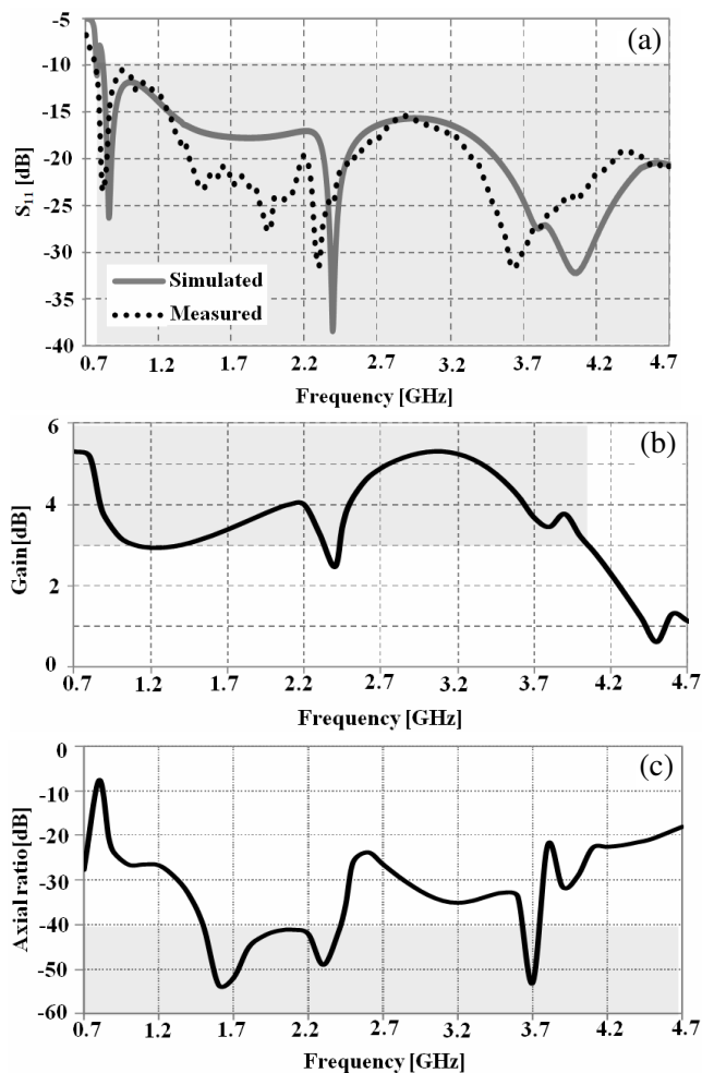
Figure 5. Parameters of the ring-loaded bowtie antenna. (a) Comparison between the simulated and the measured reflection coefficient. (b), (c) Gain and axial ratio calculated along the z direction by means of full-wave simulations performed with CST-Microwave Studio.
