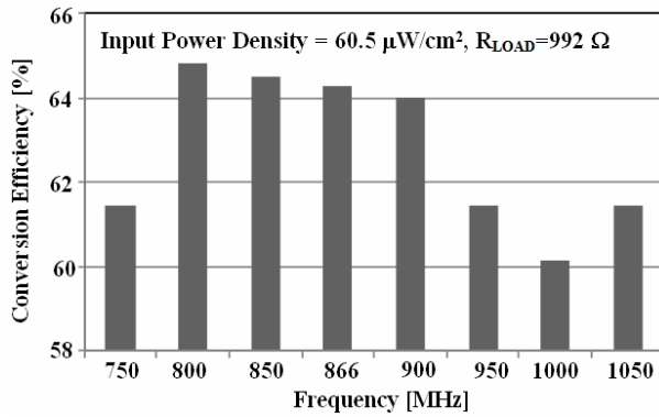
Figure 10. Measurements of \eta_{\text{RFtoDC, rectenna}} for different values of the frequency of the RF input signal.
