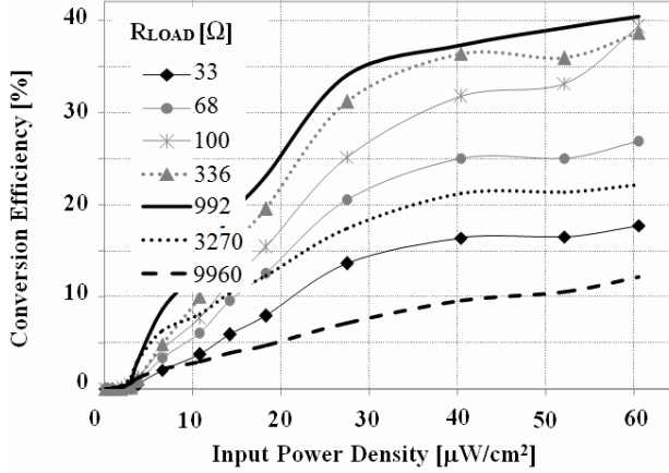
Figure 8. Measurements of \eta_{\text{RFtoDC, rectifier}} calculated by using the effective area of the antenna measured at 866 MHz.
