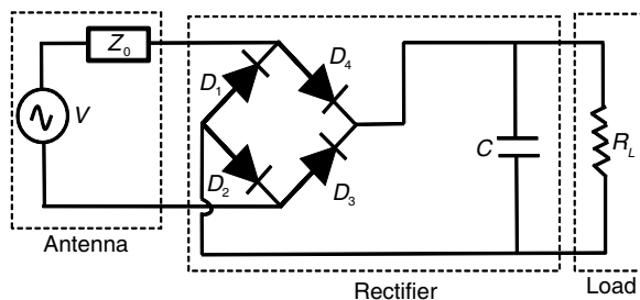
Figure 2. Lumped-element equivalent circuit of the proposed rectenna.
