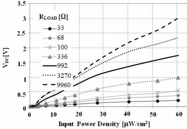
Figure 9. Measurements of the DC output voltage as function of the input power for different values of the resistive load.
