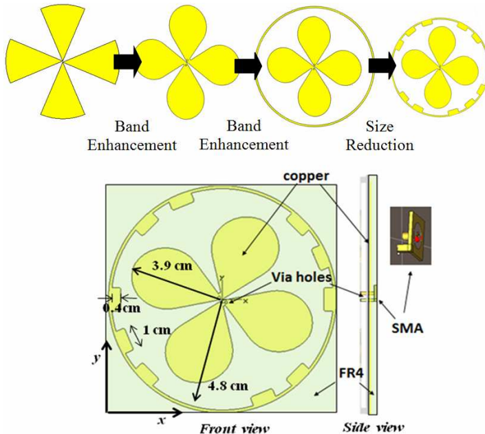
Figure 4. Design process and dimensions of the antenna.
