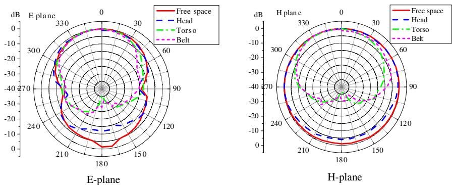
Figure 7. Normalized peak to peak voltage in dB vs. azimuth in degrees.
