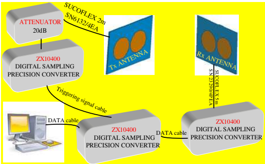
Figure 2. Time domain antenna measurement setup.
