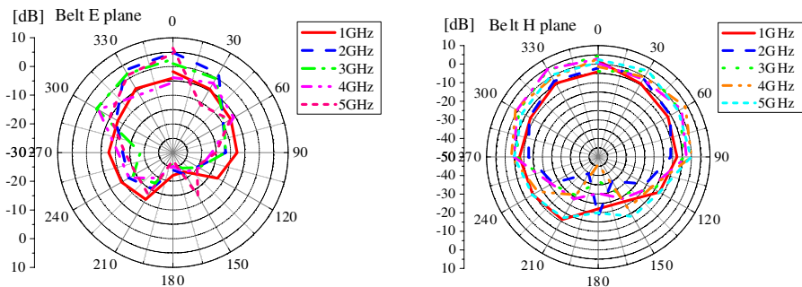
Figure 9. Radiation patterns at selected frequencies, belt scenario, E and H planes.
