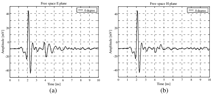
Figure 4. Measured waveforms. Antenna in a free space on a 3 m distance: (a) horizontal polarization and (b) vertical polarization.
