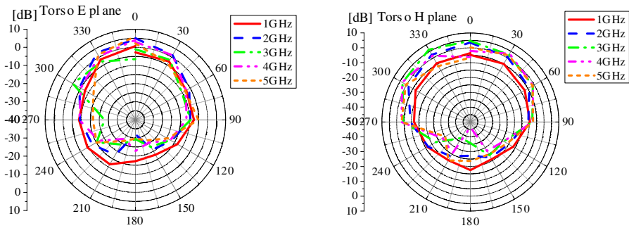
Figure 10. Radiation patterns at selected frequencies, torso scenario, E and H planes.
