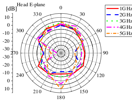
Figure 8. Radiation patterns at selected frequencies, head scenario, E plane.
