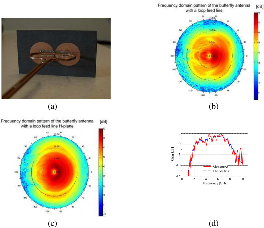
Figure 1. (a) Butterfly antenna with loop feeding, (b) measured radiation pattern: E -plane, (c) H -plane and (d) comparison theoretical/measured antenna gain.
